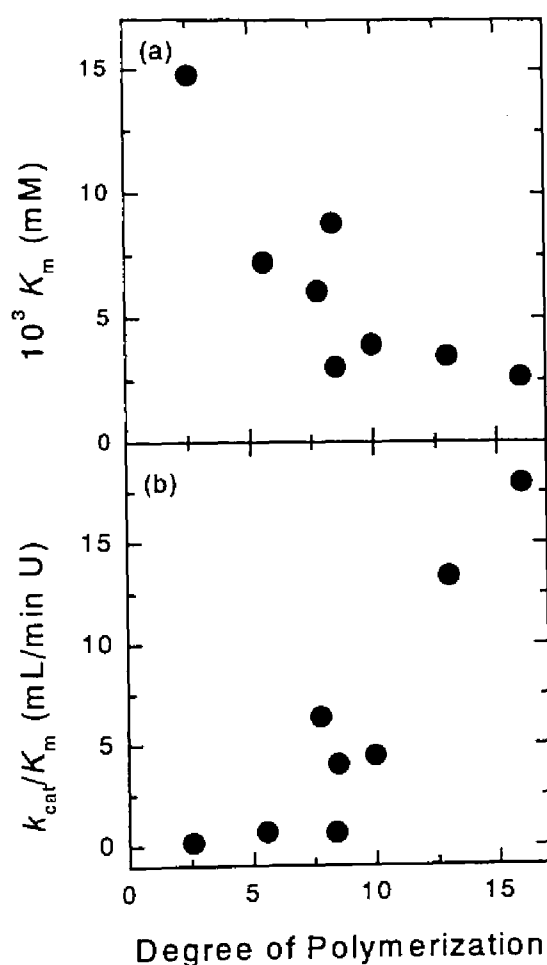
Figure 3-4. Effect of the degree of polymerization of DODA-PMEGal on K_m and k_{\text{cat}}/K_m values at 25 °C. [Enzyme] = 0.25 units/mL.
