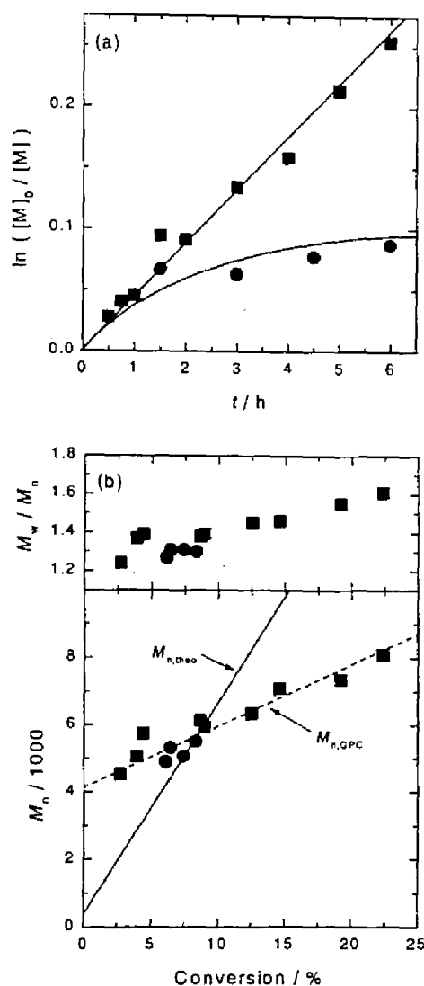
Figure 5-2. (a) Plot of \ln([M]_0/[M]) vs t and (b) values of M_n and M_w/M_n as a function of monomer conversion; solution polymerization of AIpGlc (60 wt.%) in p -xylene at 100 °C: [AIPGlc]_0/[BS-DBN]_0/[DCP]_0 = 200/1/2.4 (■) and 200/1/0 (●). The full line in Figure 5-2b represents the theoretical prediction.
