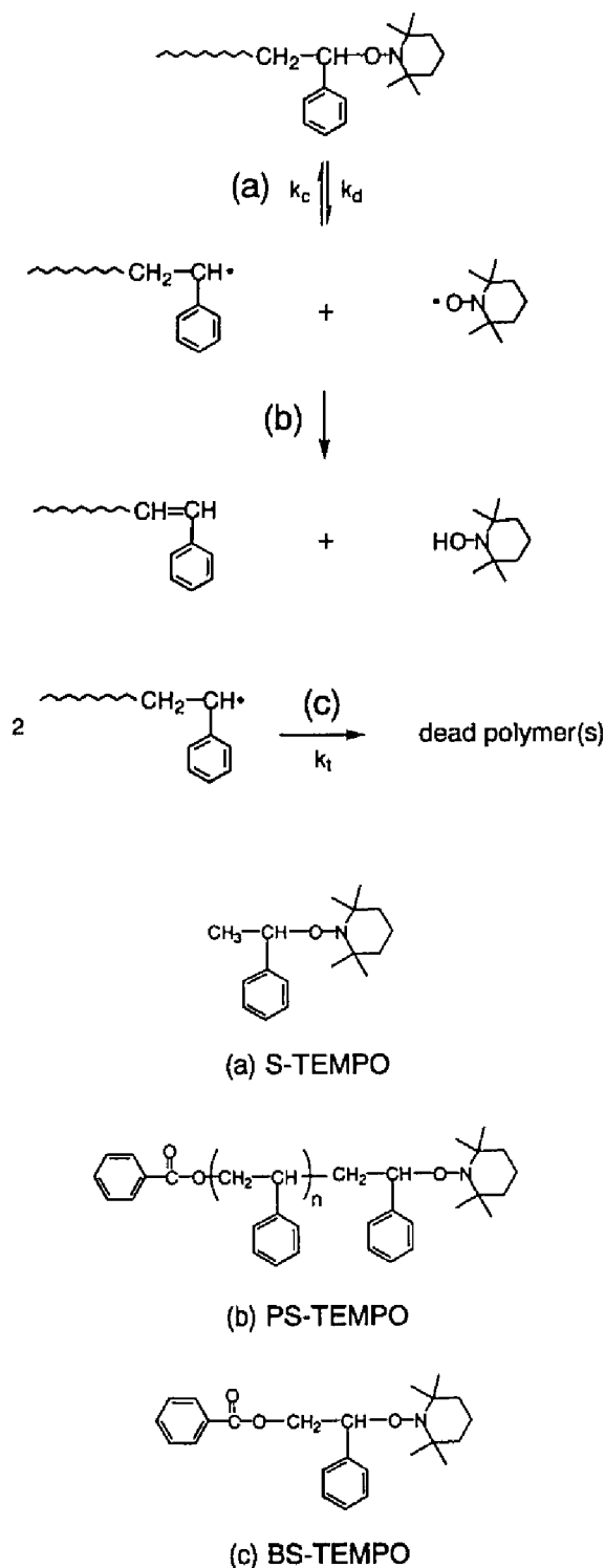
Figure A1-1. Chemical structures of (a) S-TEMPO, (b) PS-TEMPO, and (c) BS-TEMPO
