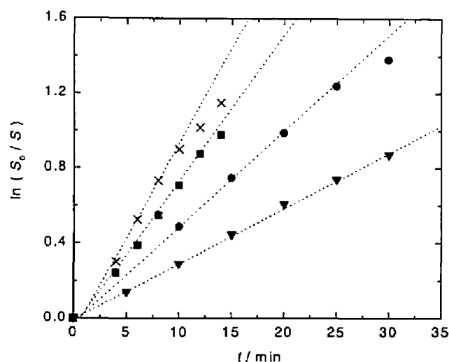
Figure A2-3. Plot of \ln(S_0/S) vs t for the PS-Br activated by cuprous halide complex at 110^\circ\text{C} : [\text{Cu(I)Br}/2\text{L}]_0 = 1 ( \blacktriangledown ), 2 ( \bullet ), 3 ( \blacksquare ), and 4 ( \times ) \text{mmol L}^{-1} .
