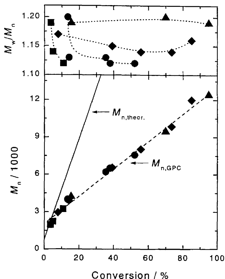
Figure 7-4. Values of M_n and M_w/M_n as a function of monomer conversion for the solution polymerization of Ac-VLA (55 wt.%) in 1,2-dichloroethane at 90 °C: [Ac-VLA] 0 /[DODA-PE-DBN] 0 /[DCP] 0 = 50/1/0 (■); 50/1/2 (●); 50/1/3 (◆), 50/1/4 (▲). The full line in the figure represents the theoretical prediction.
