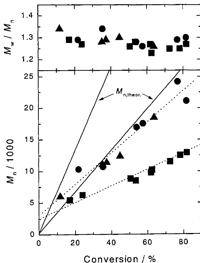
Figure 6-4. Values of M_n and M_w/M_n as a function of monomer conversion for the solution polymerization of MAIpGlc (50 wt.%) in veratrole at 80 °C: [MAIpGlc]_0/[2-(EtB)Br]_0/[Cu(I)Br]_0/[dHbipy]_0 = 100/1/0.5/1 (■); 200/1/1/2 (●); 200/1/0.5/1 (▲). The full lines in the figure represent the theoretical predictions.
