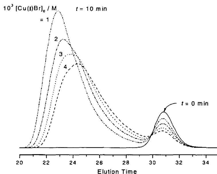
Figure A2-2. GPC charts for the PS-Br ( P_0 -X)/styrene/BHP mixture with different Cu(I)Br/2L concentrations heated at 110 °C for 10 min: [P_0\text{-X}]_0 = 12 \text{ mmol L}^{-1} ; [\text{BHP}]_0 = 20 \text{ mmol L}^{-1} ; [\text{Cu(I)Br/2L}]_0 = 1, 2, 3, \text{ and } 4 \text{ mmol L}^{-1} .
