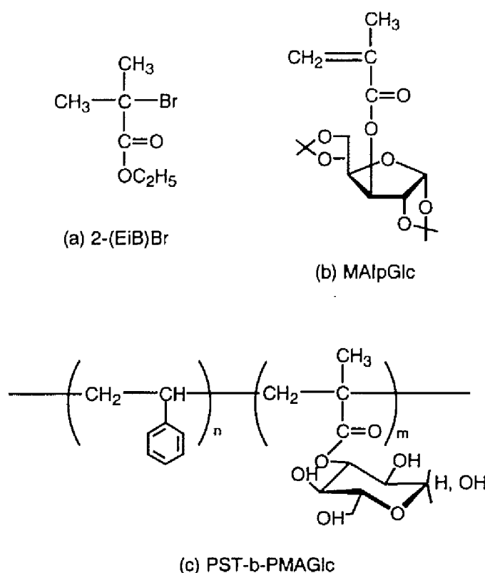
Figure 6-1. Chemical structures of (a) 2-(EtB)Br, (b) MAIpGlc, and (c) PS- b -PMAGlc.
