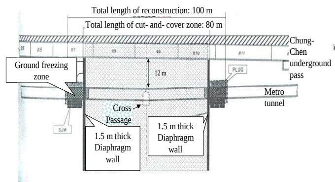
Fig. 6 Cross section of excavation in longitudinal direction
