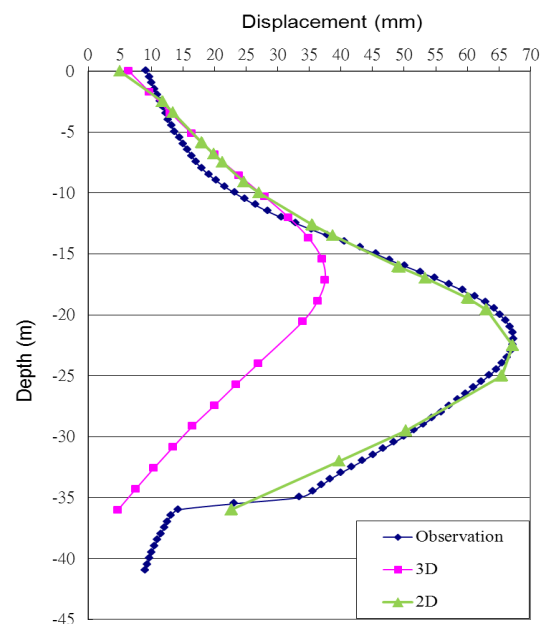
Fig. 9 Analytical wall deflections
