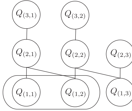
図 3: MIS-localization
