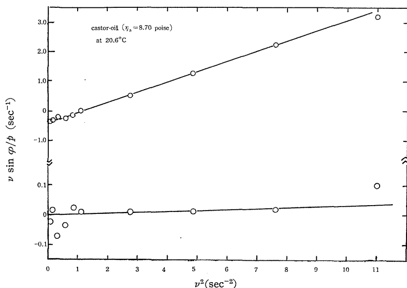
Fig. 3. Plots of \nu \sin \varphi/p and 1-\cos \varphi/p versus \nu^2 in a castor oil ( \eta_s=8.70 poise) at 20.6°C. Circles indicate the obtained data, and lines are calculated by Eqs. (3a) and (3b).
