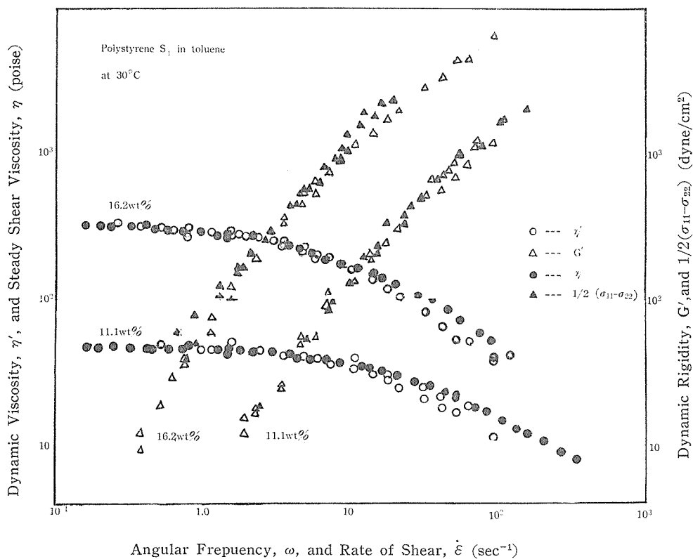
Fig. 5b. Comparison of dynamic data with steady shear data: polystyrene Th 1 in toluene at 30°C.
