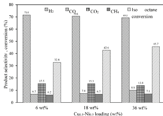
Figure 10. Effect of Ni_{0.5}-Cu_{0.5}/Al_2O_3 catalysts on conversion and product selectivity with varying Ni_{0.5}-Cu_{0.5}/Al_2O_3 ratios: T = 550 \text{ °C} ; N_2 = 15 \text{ cm}^3/\text{min} , iso -octane feed rate was 0.03 g/min; S/C molar ratio: 0.9.
