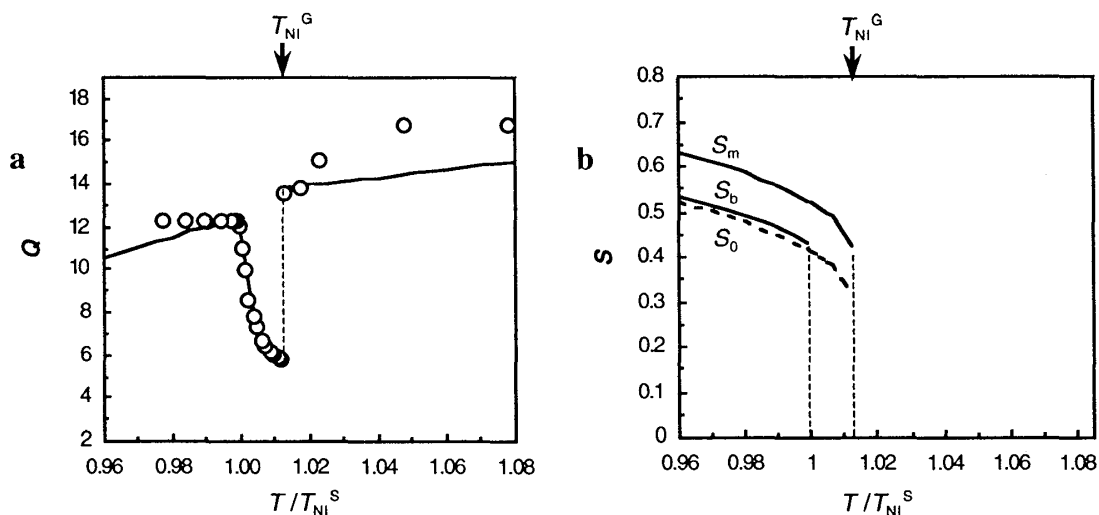
Fig. 1. (a) Degree of equilibrium swelling of a LC gel in a nematic solvent as a function of reduced temperature. The temperature is reduced by the nematic-isotropic temperature of the nematic solvent outside the gel ( T_{\text{NI}}^{\text{S}} ). The solid line represents the prediction of a mean-field theory. (b) Orientational order parameters of mesogen on gel, nematic solvents inside and outside the gel ( S_m , S_0 , S_b , respectively) as a function of reduced temperature calculated using the mean-field theory with the same parameter values as (a).
