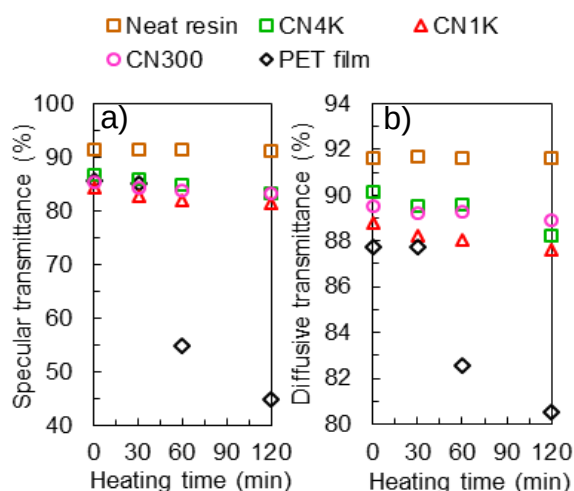
Figure 4.12. Optical transmittance at 600 nm wavelength as a function of the heating time at 180 °C.
