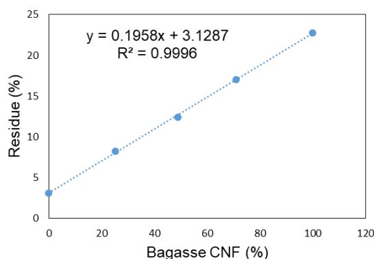
Figure 3.1. TGA-residue versus bagasse CNFs graph with the regression equation to determine the CNF-content of the nanocomposites. TGA was performed by placing approximately 5–10 mg mixture of the dried-CNFs and cured-resin of known composition on a platinum pan, stabilized at 110 °C for 10 min to remove residual moisture, and analyzed from 110 to 600 °C at a heating rate of 10 °C min -1 under a nitrogen flow rate of 100 ml min -1 .
