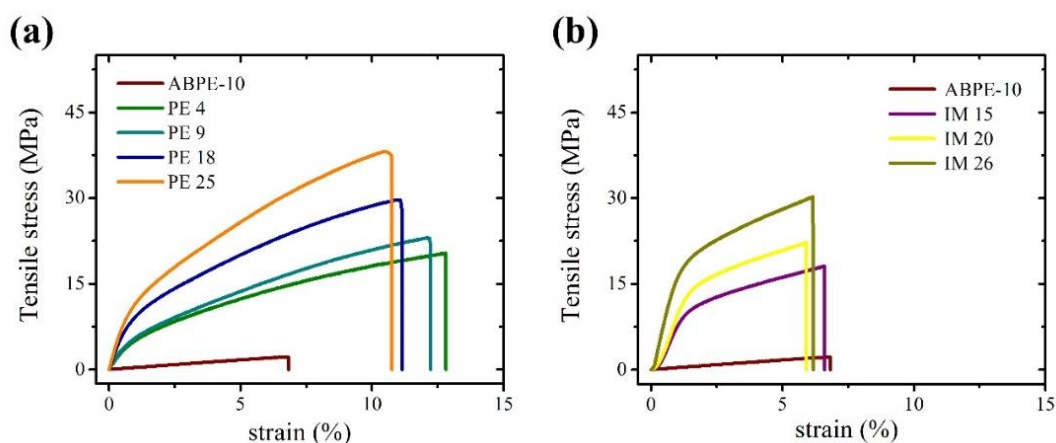
Figure 3.7. Tensile stress-strain curves of the CNF-reinforced nanocomposites prepared by (a) Pickering emulsification method and (b) impregnation method.
