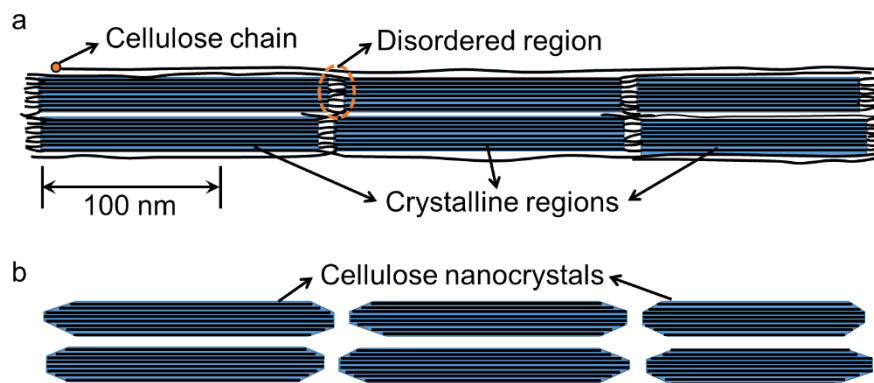
Figure 1.2. (a) Model CNFs with the semi-crystalline configuration, and (b) CNCs that can be retrieved after the removal of amorphous (disordered) regions via acid hydrolysis [2]. Adapted with permission from ref. 2 © 2011 The Royal Society of Chemistry.
