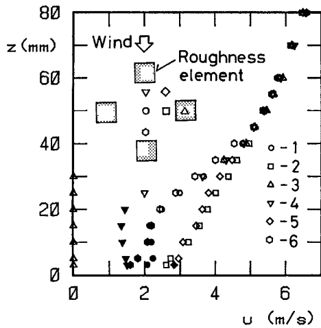
Fig. 7a. Mean wind speed profiles at various locations (CASE B410).
