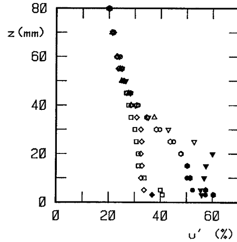
Fig. 7b. X-component turbulence intensity profiles at various locations (CASE B410).
