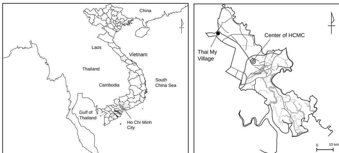
Figure 3-1 Location of Ho Chi Minh City and Thai My Village
