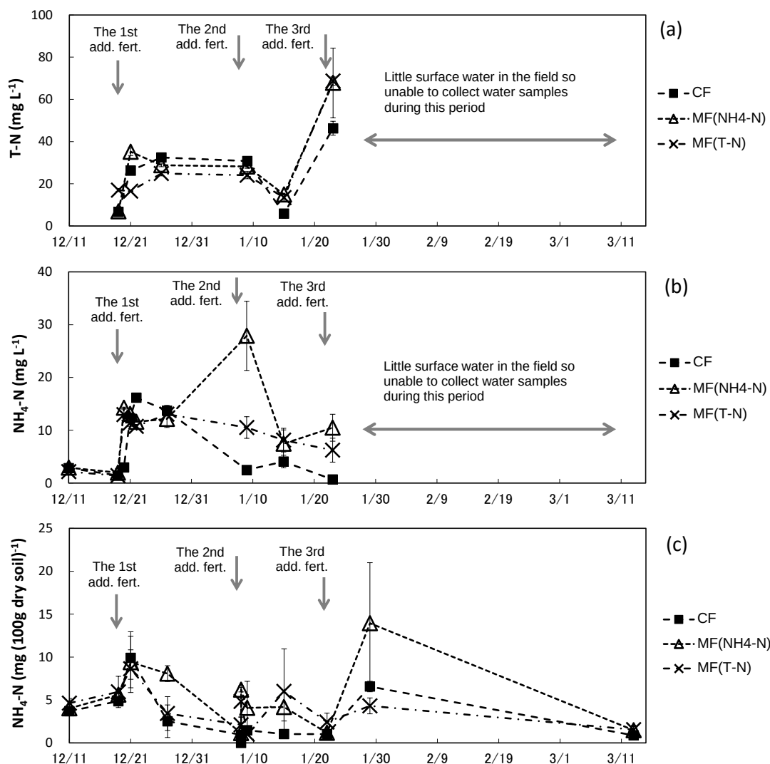
Figure 4-4 (a) T-N in surface water, (b) NH 4 -N in surface water, (c) NH 4 -N in surface soil (n=2)
