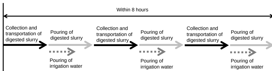
Figure Ap2-1 Sequence in 8 hours for slurry fertilization with 400 \text{ mg L}^{-1} of T-N
