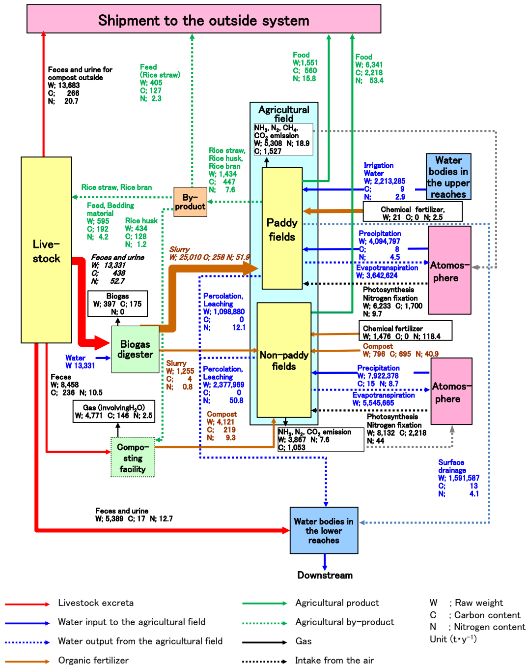
Figure 6-1 “Scenario 1” based on the scenario for increasing biogas digesters and using the slurry from them in paddy fields
