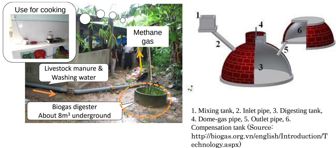
Figure 2-1 Fixed dome type of household biogas digester
