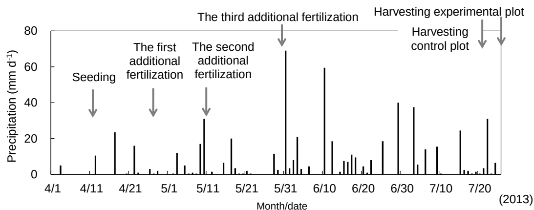
Figure 5-7 Precipitation during cultivation
