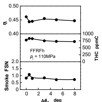
Fig.4 Effects of dwell between 3rd and 4th injection stages on thermal efficiency and exhaust emissions
