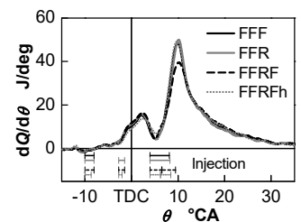
Fig.2 Heat release rates (3- and 4-stages injection)
