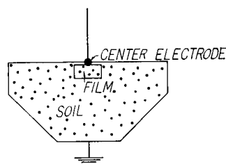
Fig. 1. Arrangement of center electrode and embedded film in the vessel filled with soil.
