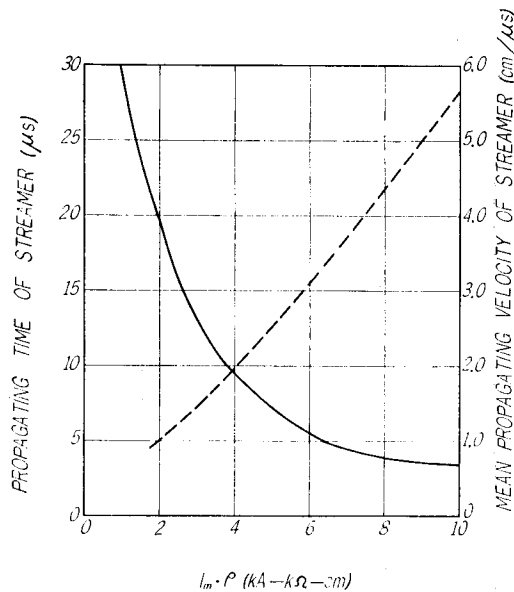
Fig. 25. Mean propagating velocity against I_m \cdot \rho
