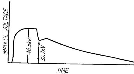
Fig. 26. Potential drop between gap in soil against elapsed time.
