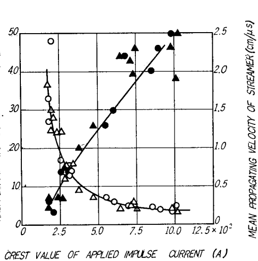
Fig. 16. Mean propagating velocity of streamer.
