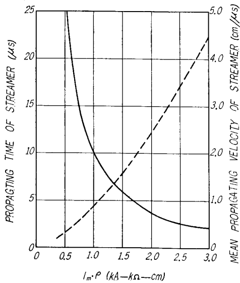
Fig. 23. Mean propagating velocity against I_m \cdot \rho .
