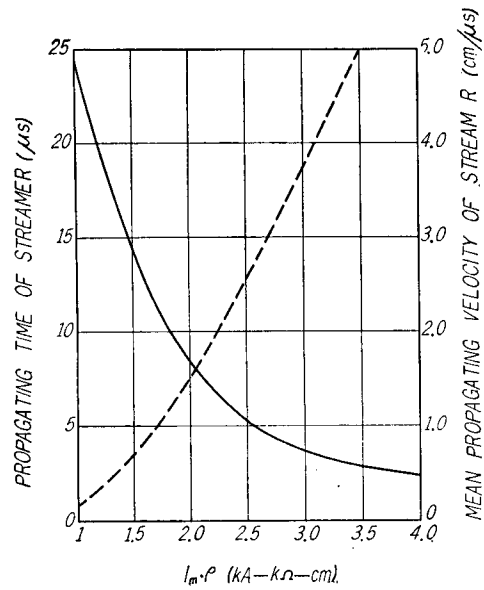
Fig. 24. Mean propagating velocity against I_m \cdot \rho .
