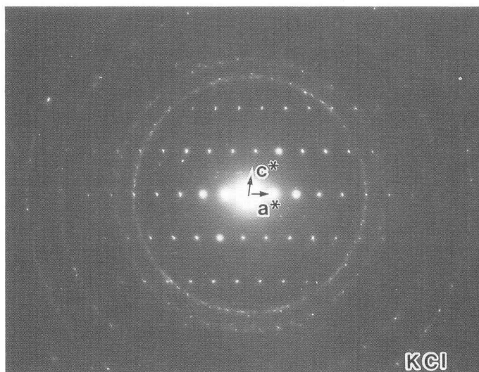
Fig. 2. Electron diffraction pattern taken from PbPc grown on KCl at 200°C. The diffraction pattern corresponds also to the \mathbf{a}^*\mathbf{c}^* -net pattern of the triclinic form. The ring patterns come from gold crystallites deposited on a microgrid frame.
