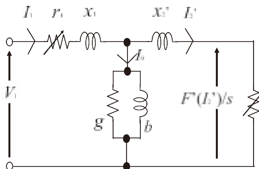
Fig. 1. Schematic diagram of equivalent circuit of the fully superconducting HTS-ISM
