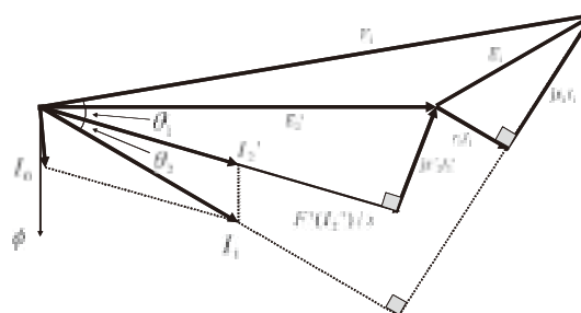
Fig. 2. Phasor diagram of the HTS-ISM
