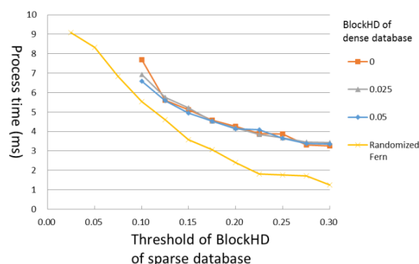
Fig.6 Process time of 2-step Randomized Fern
