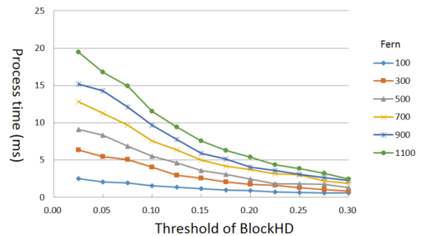
(b) Process time with respect to threshold of BlockHD
