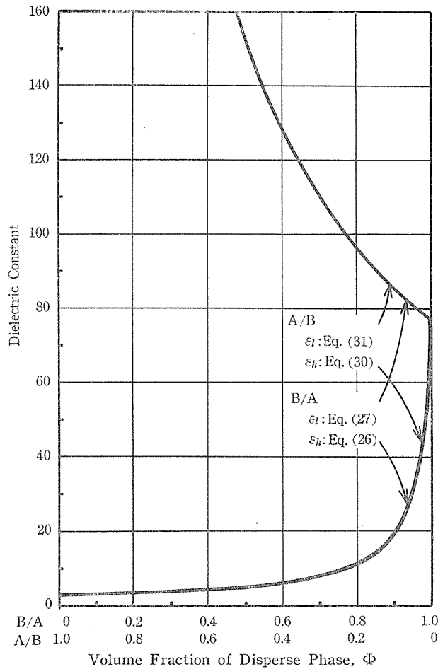
Fig. 8. Concentration dependence of dielectric constants \varepsilon_h and \varepsilon_l for the A-in-B and the B-in-A emulsions given by the Maxwell theory.
