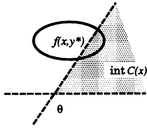
Fig.1: f(x, y^*) \notin \text{int } C(x).
