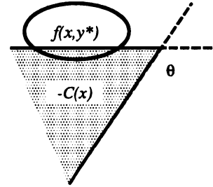
Fig.3: f(x, y^*) \cap (-C(x)) \neq \emptyset.
