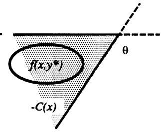
Fig.4: f(x, y^*) \subset (-C(x)).
