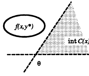
Fig.2: f(x, y^*) \cap \text{int } C(x) = \emptyset.
