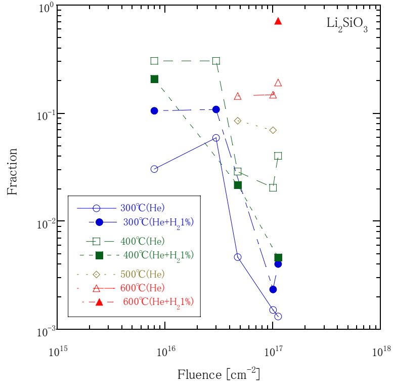
Fig. 2-4. Neutron fluence dependence of the total yield y_2^\infty of HTO released with the reaction controlled kinetics in isothermal annealing experiments of Li 2 SiO 3 .
