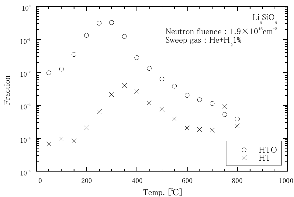
Fig. 2-2. Typical tritium release behaviors from \text{Li}_4\text{SiO}_4 observed in annealing experiments with a constant heating rate of 5K/min.
