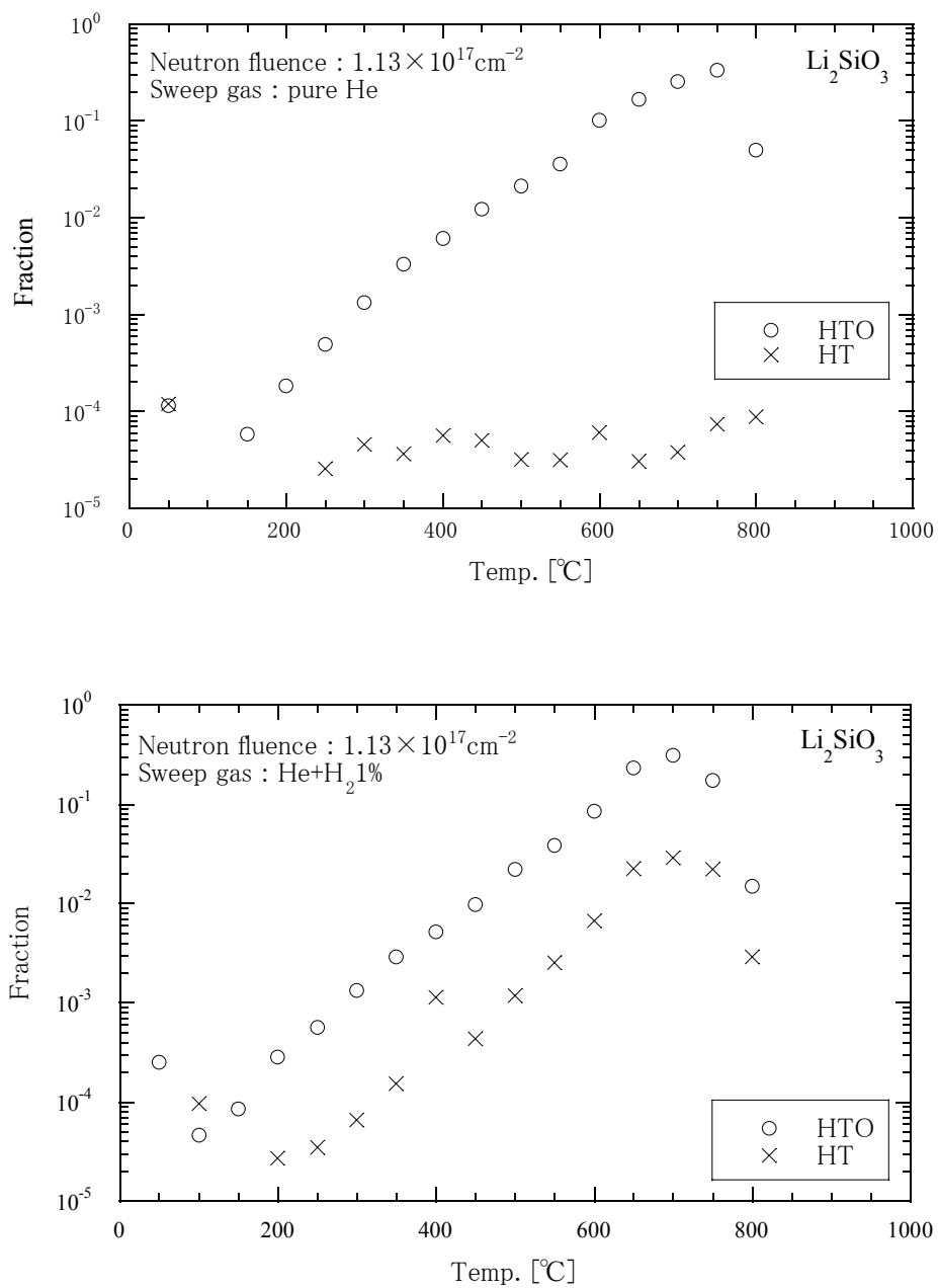
Fig. 2-1 (cont'd). Typical tritium release behaviors from Li 2 SiO 3 observed in annealing experiments with a constant heating rate of 5K/min.
