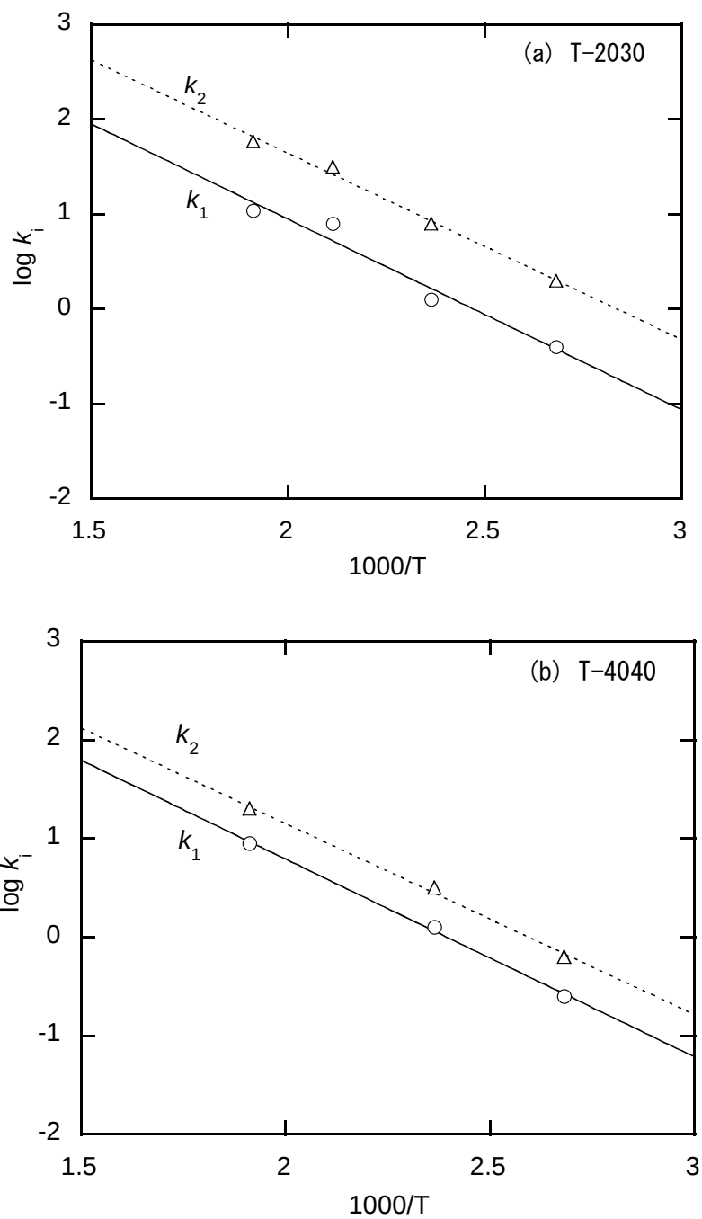
Fig. 5-14. Arrhenius plots of reaction rate constant k_1 and k_2 for (a) T-2030 and (b) T-4040. Marks are experimental and curves represent the least-squares fits of the data to the Arrhenius equations.
