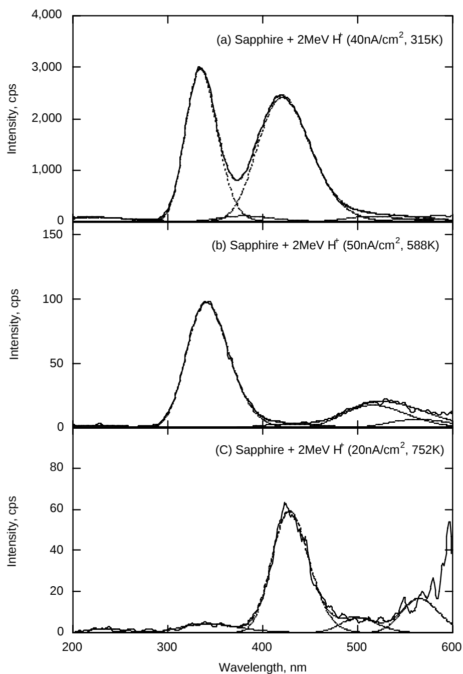
Fig. 4-2. Typical luminescence spectra of sapphire under 2MeV H^+ ion beam irradiation. The ordinate represents luminescence intensity normalized to the beam current of 10\text{nA/cm}^2 . Curves represent the results of decomposition as described in 4.3.1.
