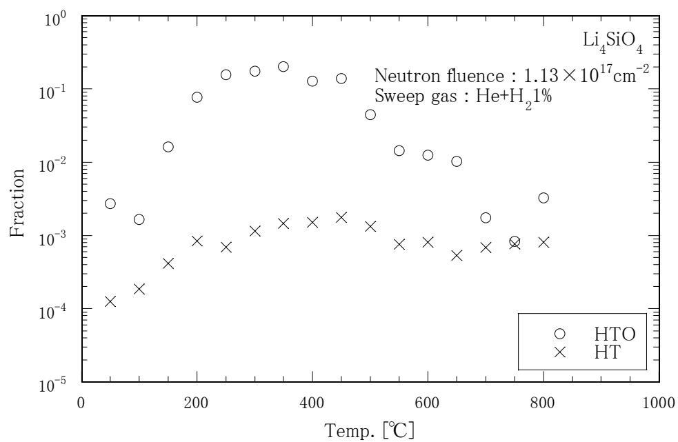
Fig. 2-2 (cont'd). Typical tritium release behaviors from \text{Li}_4\text{SiO}_4 observed in annealing experiments with a constant heating rate of 5K/min.
