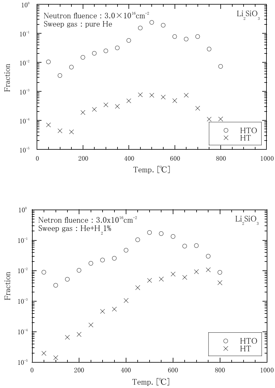
Fig. 2-1. Typical tritium release behaviors from Li 2 SiO 3 observed in annealing experiments with a constant heating rate of 5K/min.
