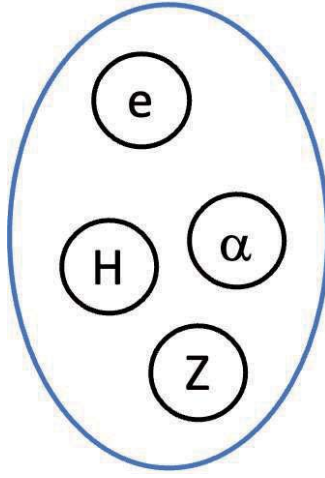
Fig. 4: Plasmas with multiple ion components. In practice, plasmas contain electrons ( e ), fuel ions (usually hydrogen, H ), fusion products ( \alpha particle), and impurities ( Z , Carbon, Tungsten, etc).
