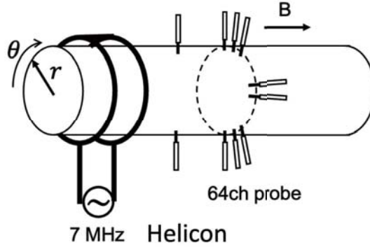
Fig. 3: A schematic diagram for the experimental device, PANTA.
