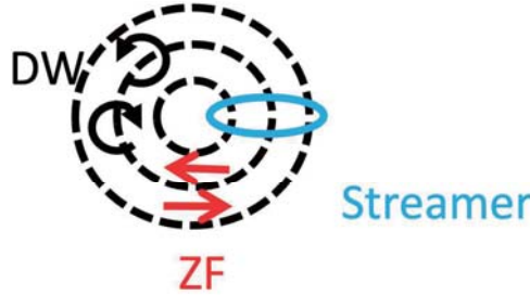
Fig. 2: The cross section of a cylindrical magnetized plasmas. Small scale drift wave turbulence nonlinearly interact with each other to pump large scale flows, such as zonal flows or streamers. Zonal flows are purely azimuthal with the radial variation, while streamers are radially elongated and azimuthally localized.
