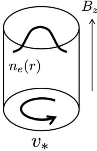
Fig. 1: A plasma of interest. Magnetic field is imposed in the axial direction. Plasma has inhomogeneity in the radial direction. For simplicity, only density field is considered. The density gradient drives drift waves, which propagate in the azimuthal direction at the drift speed v_* .
