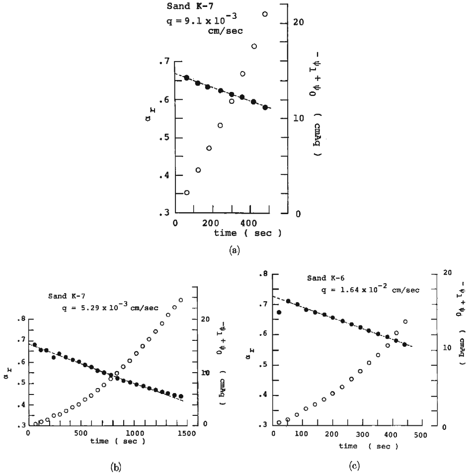
Fig. 12 Changes of \alpha_r and (-\psi_1 + \psi_0)
