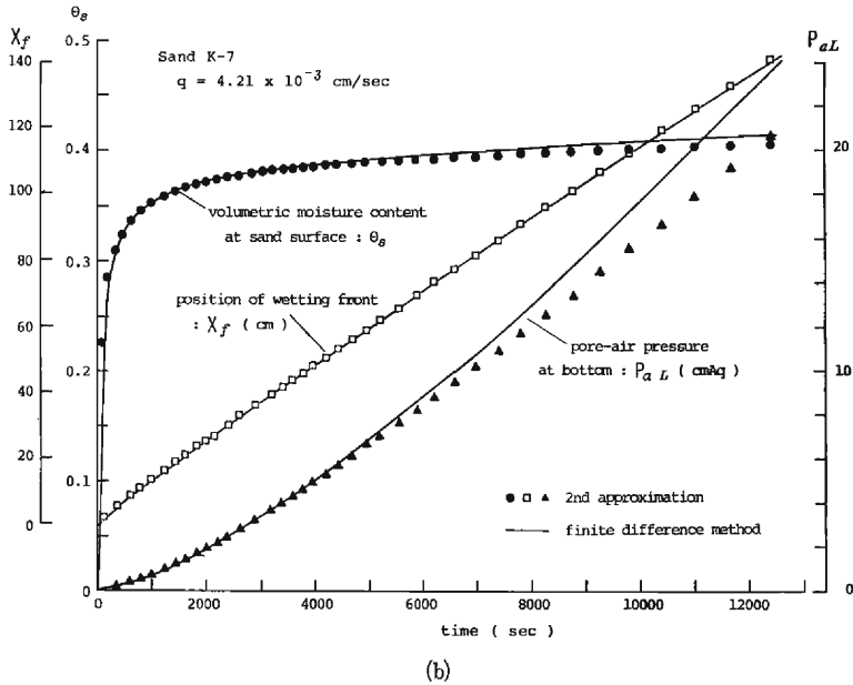
Fig. 2 Comparison of the calculated values by approximate solution with ones by finite difference method
