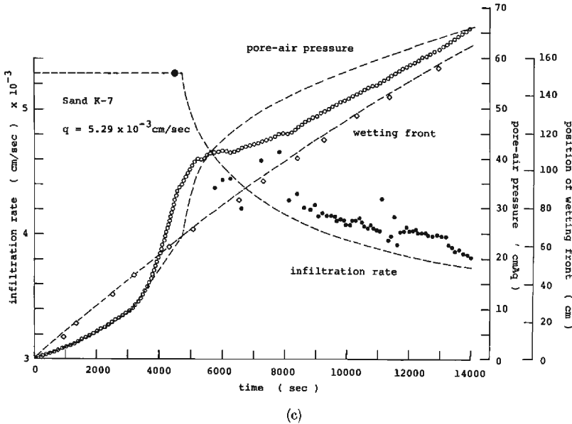
Fig. 18 Changes of the depth of wetting front, the infiltration rate and the pore-air pressure ahead of wetting front in the case of Sand K-7
