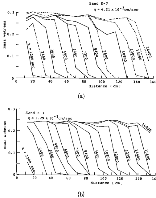
Fig. 16 Change of observed moisture profile (a) in the case of Fig. 15 (a) (b) in the case of Fig. 15 (b)
