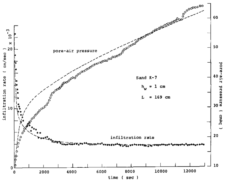
Fig. 20 Changes of the infiltration rate and the pore-air pressure at the bottom of a layer in ponded infiltration
