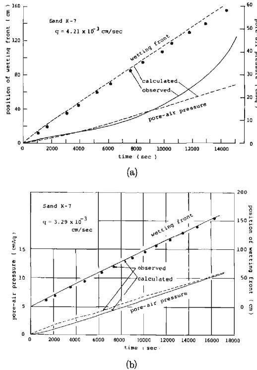
Fig. 15 Changes of the pore-air pressure and the depth of wetting front in the case of Sand K-7 (a) q = 4.21 \times 10^{-3} cm/sec (b) q = 3.29 \times 10^{-3} cm/sec
