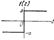
Fig. 9. The on-off relay characteristic.
