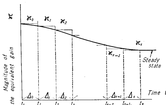
Fig. 4. Equivalent gain when the time t is divided into contiguous disjointed intervals of \Delta_j = t_{j+1} - t_j .
