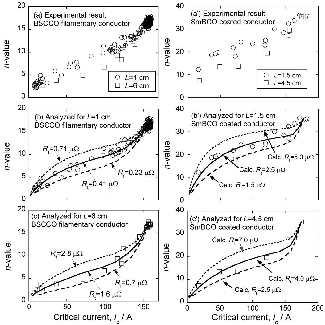
Fig. 9 Examples of specimen length-dependence of experimentally measured n-I_c diagrams and the results analyzed by the upper-lower bounds approach for filamentary- and coated- conductor tapes. (a) and (a') show the experimental results of BSCCO filamentary tape for L = 1 cm and 6 cm 15) and SmBCO coated tape for L = 1.5 cm and 4.5 cm 8) , respectively. (b) and (c) show the analyzed results of BSCCO filamentary tape for L = 1 cm and 6 cm, respectively. (b') and (c') show the analyzed results of SmBCO coated tape for L = 1.5 cm and 4.5 cm, respectively.
