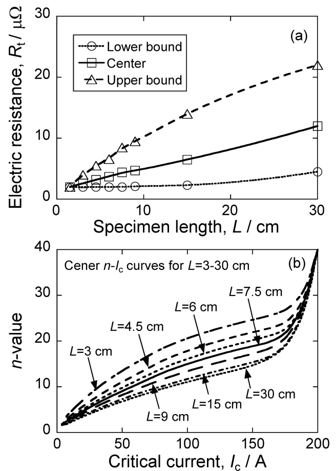
Fig. 8 (a) Change in R_t -value with increasing specimen length L for the upper-lower bounds and the center. (b) Change in the n-I_c relation of the center in the n-I_c diagram with increasing L , calculated with the R_t -values shown in (a) ( R_t = 2.6, 3.2, 3.7, 4.4, 4.7, 6.5 and 12.0 \mu\Omega for L = 3, 4.5, 6, 7.5, 9, 15 and 30 cm, respectively). In (b), the n-I_c curves for the center are taken up representatively from the n-I_c curves calculated for the upper-lower bounds and the center.
