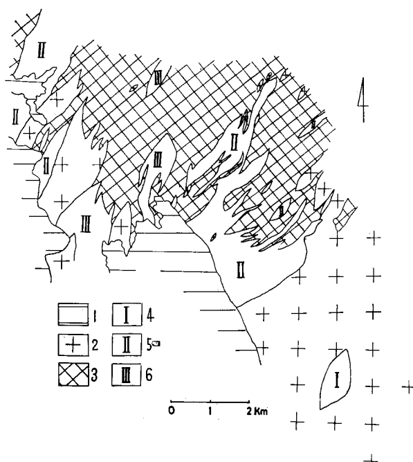
Fig. 5. Zones of progressive metamorphism in the Toyone-mura area.
