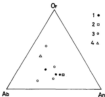
Fig. 3. Triangular diagram showing the ratios of normative orthoclase (Or), albite (Ab) and anorthite (An) of the granitic rocks of the Toyone-mura area. 1: Kamihara granite 2: Tashika granite 3: Mitsuhashi granite 4: Busetsu granite
