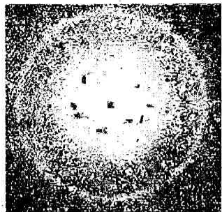
Fig. 4. Annealed at 500^{\circ}\text{C} in the Stream of \text{H}_2 . ( L=8 cm, Mo Radiation)
