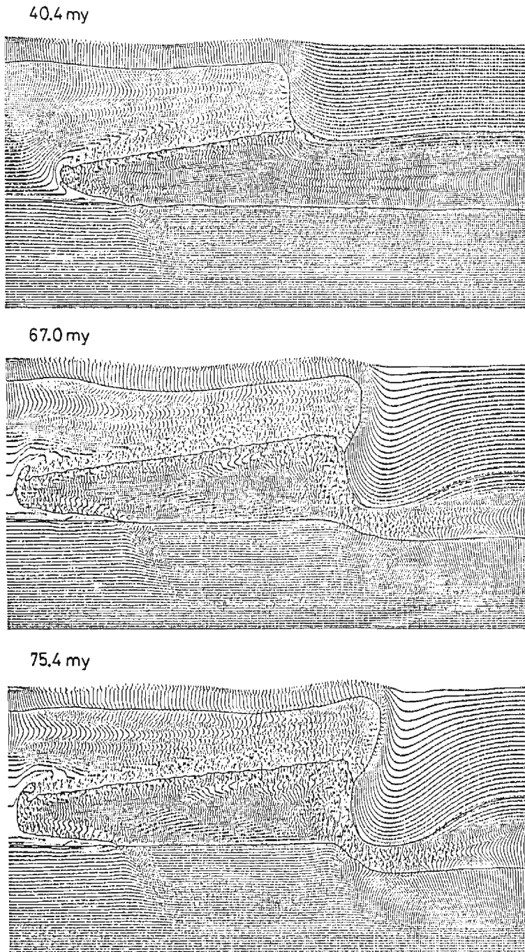
Fig. 4c Time evolution of fluid flow for Case C of Fig. 3.
