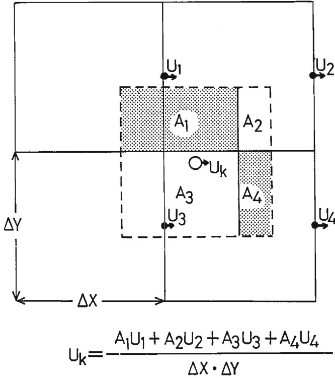
Fig. A1 Linear interpolation for the horizontal velocity, U_k , of the k -th marker particle from the velocity field U_1 to U_4 . A_1 to A_4 indicate the area of rectangular sub-regions. The interpolation for the vertical velocity V_k is performed in a similar way.
