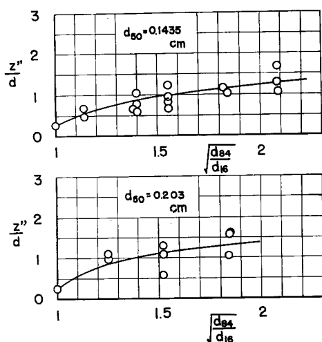
Fig. 2 Origin of coordinate for velocity profiles ( d=d_{50} )
