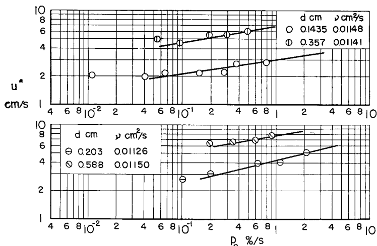
Fig. 3 Some examples of relations between rate of movement of sands and gravels, and shear velocity
