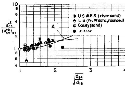
Fig. 15 Relation between u_{*c0}^{*2}/(u_{*c0}^{*2})_{0.7} and (d_{84}/d_{16})^{1/2}
