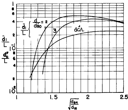
Fig. 23 Variations of \bar{d}_t/L with (d_{84}/d_{16})^{1/2}
