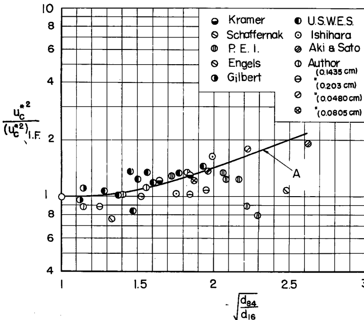
Fig. 14 Relation between u_{*c}^{*2}/(u_{*c0}^{*2})_{I.F.} and (d_{84}/d_{16})^{1/2}
