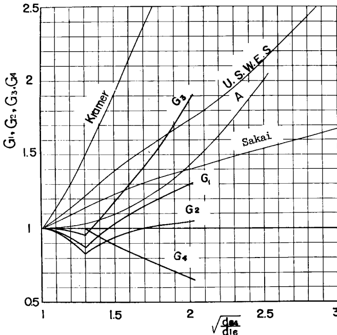
Fig. 27 Variations of G_1 , G_2 , G_3 and G_4 with (d_{84}/d_{16})^{1/2}
