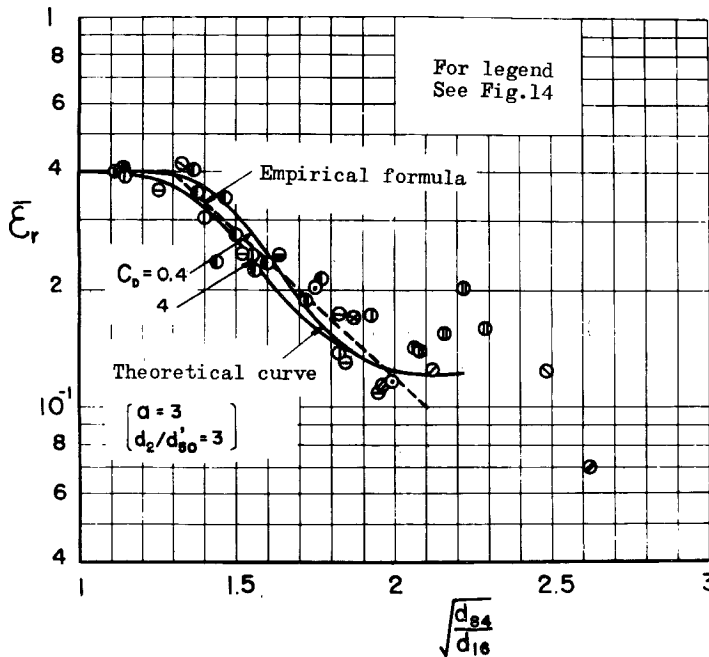
Fig. 25 Comparison of theoretical curves for sheltering coefficient and experimental results
