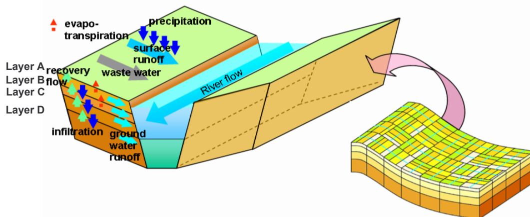
Fig.2 Schematic view of Hydro-BEAM
