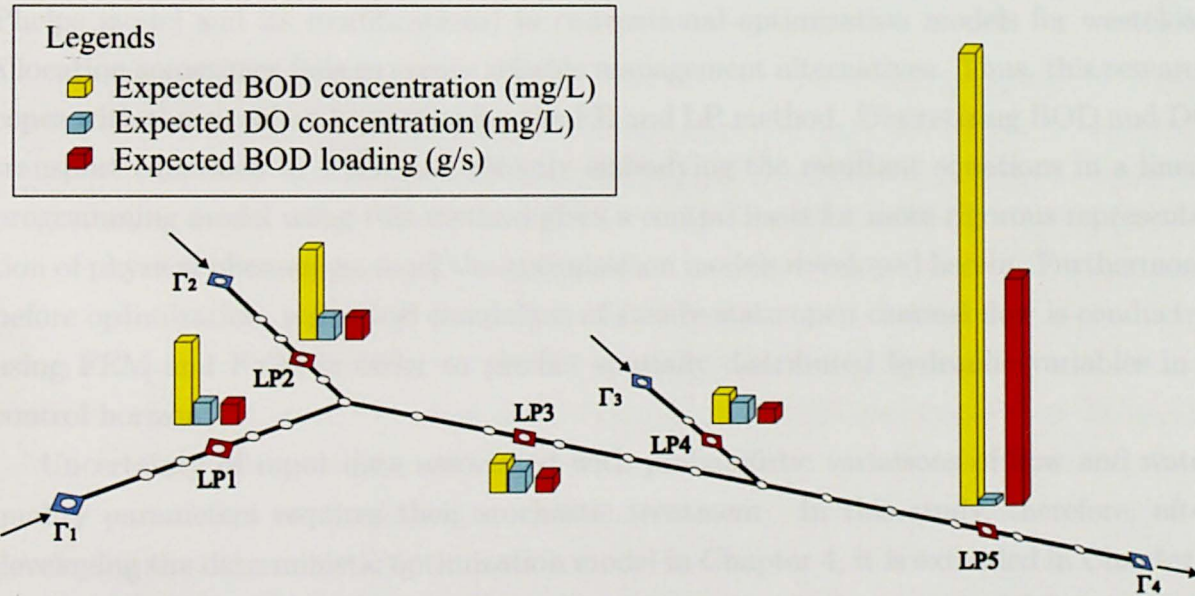
Figure 7.8: Optimal wasteload allocation in Solution D
