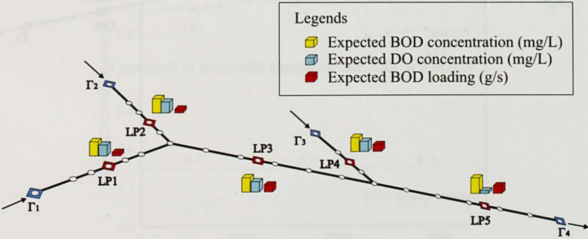
Figure 6.5: Optimal wasteload allocation in Solution D
