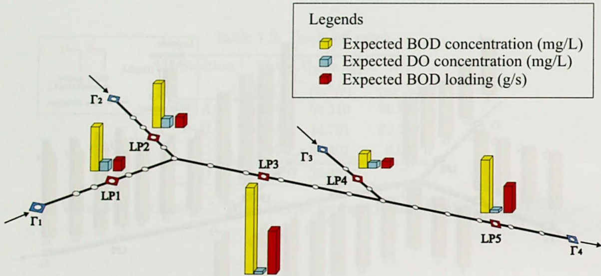
Figure 7.5: Optimal wasteload allocation in Solution A
