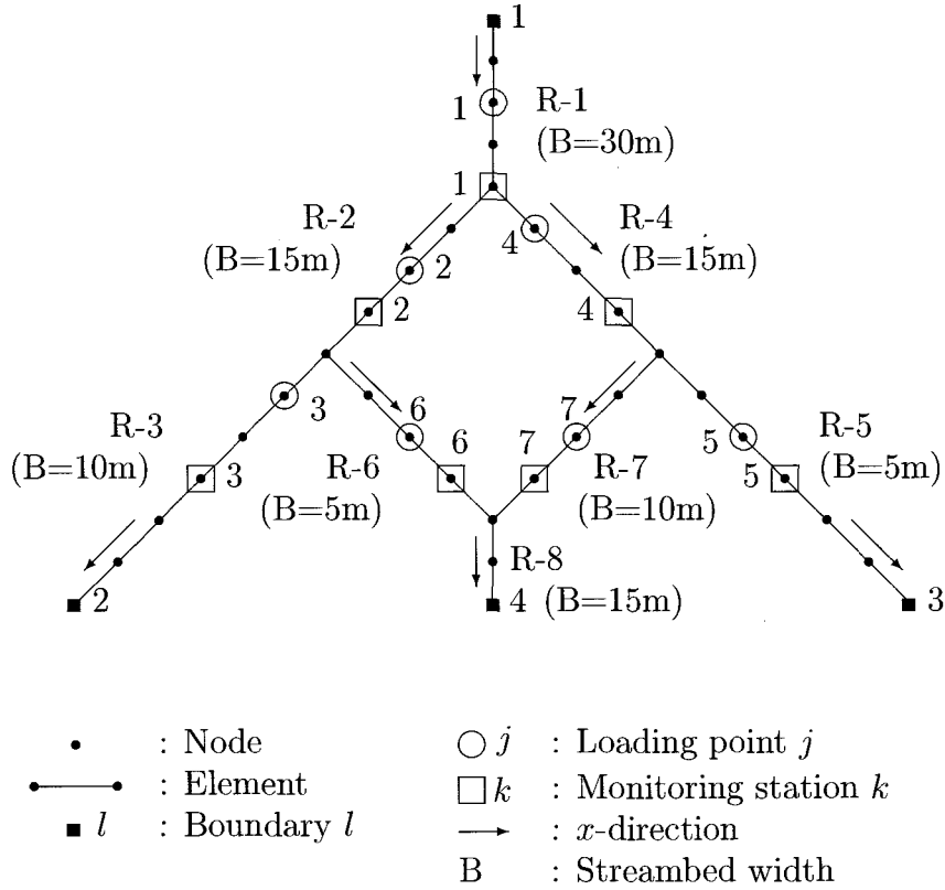
Figure 4.4: Topological sketch of stream network
