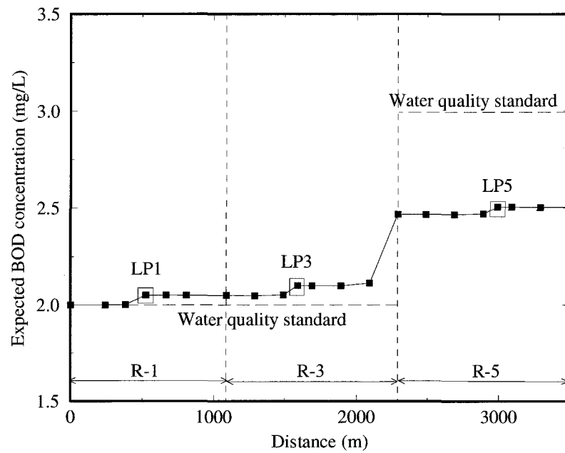
Figure 6.9: Expected BOD concentration profile of Solution D
