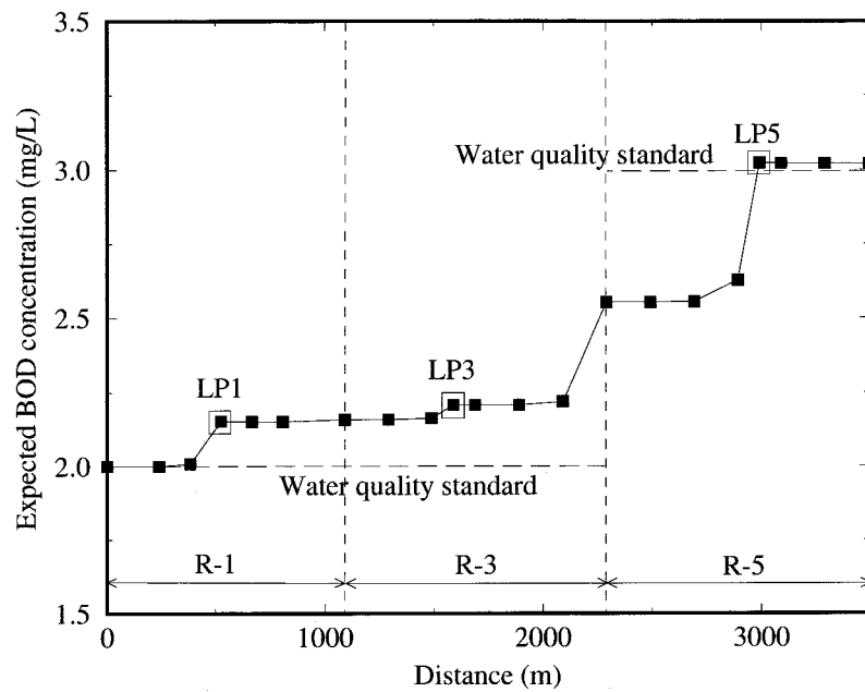
Figure 6.7: Expected BOD concentration profile of Solution A
