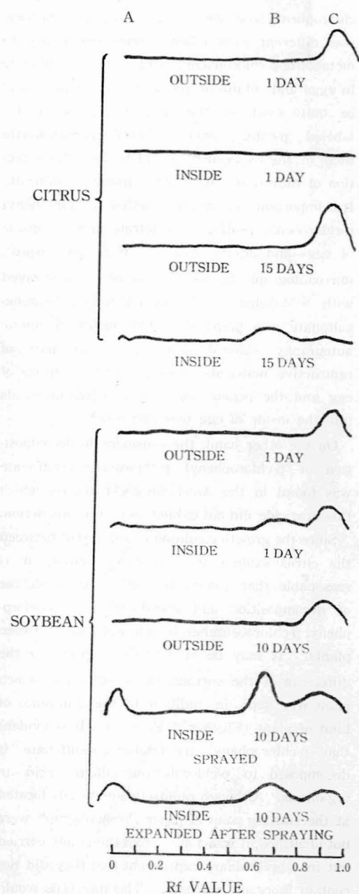
Fig. 2. Metabolism of p-chlorophenyl p-chlorobenzenesulfonate by the leaves of citrus and soybean, based on density scans of radioautographs prepared from paper chromatograms of benzene and water extracts of plants.
