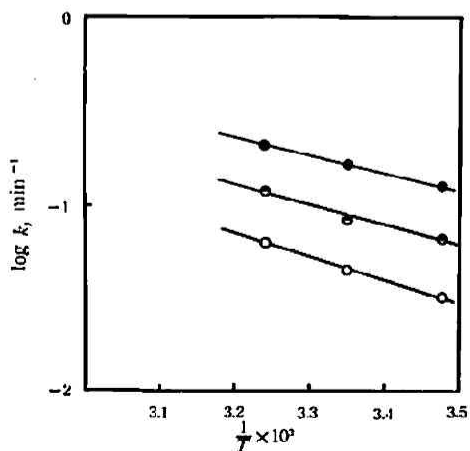
Fig. 9 Relation between logarithm of rate constant k ( \text{min}^{-1} ) and reciprocal of absolute temperature
