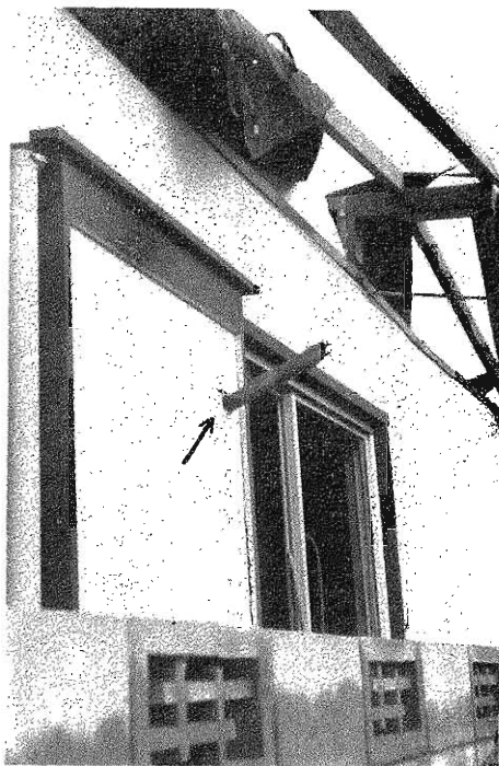
Photo. 8. Piece of wood thrust into a wall.
