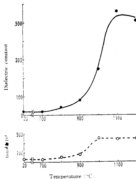
Fig. 1.5. Dependence of dielectric properties upon heating temperature for the glass No. 2.
