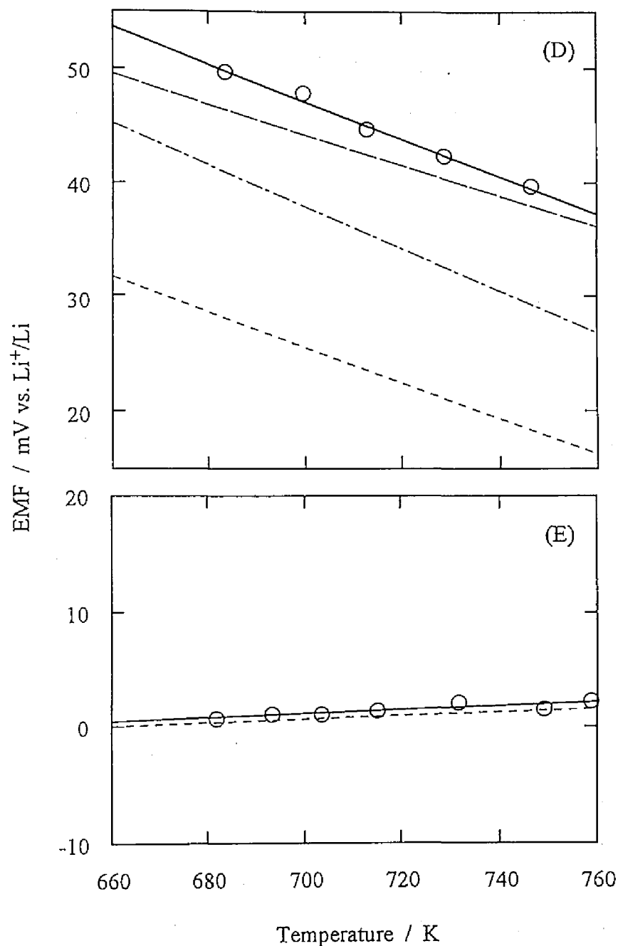
Fig.I-21. Emf as a function of temperature in the isothermal cell (I-e) with a Li-Si alloy electrode in the coexisting phase state: (A) \text{Si}+\text{Li}_{12}\text{Si}_7 , (B) \text{Li}_{12}\text{Si}_7+\text{Li}_7\text{Si}_3 , (C) \text{Li}_7\text{Si}_3+\text{Li}_{13}\text{Si}_4 , (D) \text{Li}_{13}\text{Si}_4+\text{Li}_{22}\text{Si}_4 , and (E) \text{Li}_{22}\text{Si}_5+\text{liq.} . The short-dashed line, the long-dashed line, and the dash-dotted line show the values obtained by Sharma et al. [3], Lai et al. [4] and Nikolaiev et al. [5], respectively.
