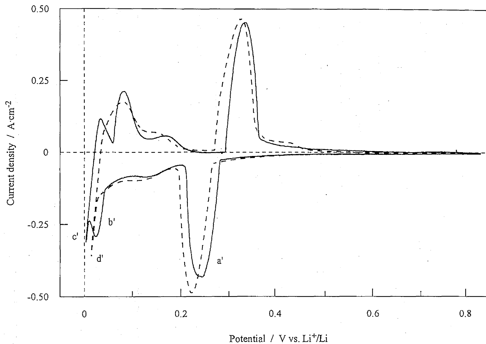
Fig.I-6. Cyclic voltammograms of an aluminum electrode in LiCl-KCl eutectic melt at 733 K (—) and 803 K (---), scan rate: 0.1 \text{ mV} \cdot \text{s}^{-1} .
