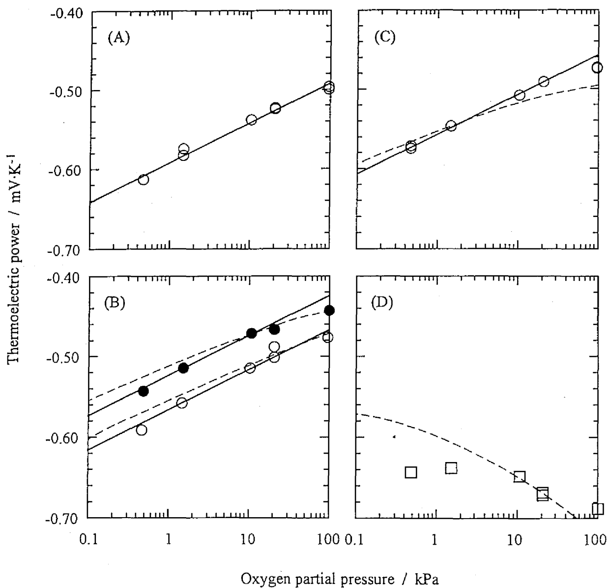
Fig.II-5. Thermoelectric power of the cell (II-b) as a function of oxygen partial pressure for (A) p_{H_2O} = 4.3 kPa at 873 K ( \bigcirc ), (B) p_{H_2O} = 4.3 kPa ( \bigcirc ) and p_{H_2O} = 1.5 kPa ( \bullet ) at 973 K, (C) p_{H_2O} = 4.3 kPa at 1073 K and (D) p_{H_2O} = 0.26 kPa at 1173 K ( \square ). The solid lines show the theoretical slope predicted by eq. (II-11). The dashed lines present the calculated values by using eq. (II-28) and (II-31).
