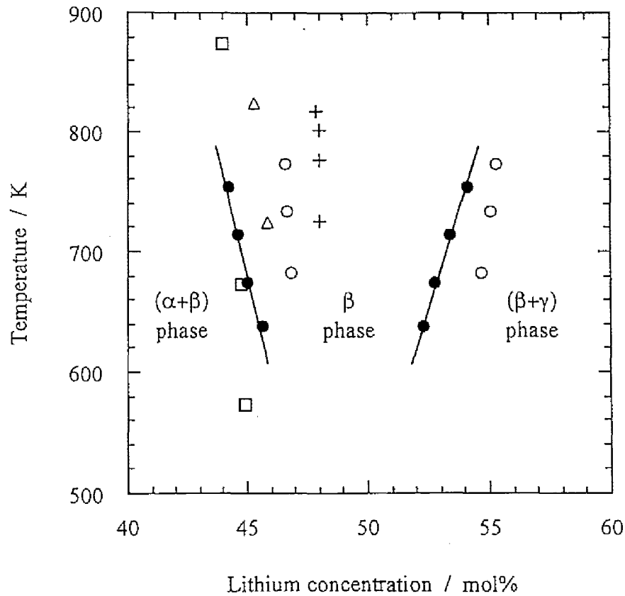
Fig.I-13. Lithium concentration range of the single \beta\text{LiAl} phase; this work (●), Wen et al. (○) [2], Levine et al. (△) [4], Veleckis (+) [5] and Schürmann et al. (□) [6].
