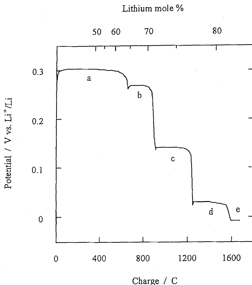
Fig.I-18. Potential transient curve of a silicon electrode in LiCl-KCl eutectic melt at 713 K. Current density; 20 \text{ mA}\cdot\text{cm}^{-2} .
