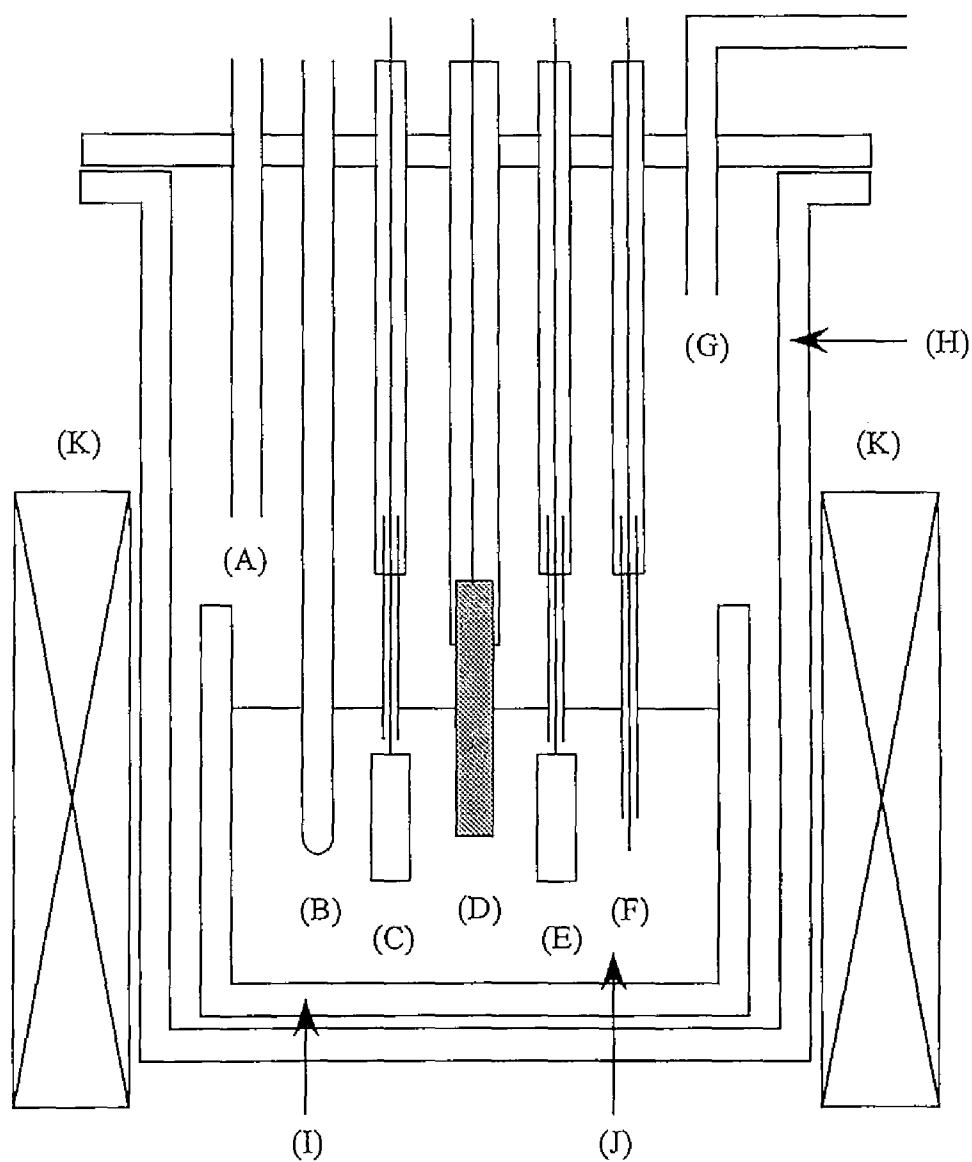
Fig.I-2. The experimental apparatus: (A) Ar gas inlet, (B) thermocouple, (C) working electrode, (D) counter electrode, (E) reference electrode, (F) \text{Li}^+/\text{Li} electrode, (G) Ar gas outlet, (H) pyrex holder, (I) crucible, (J) LiCl-KCl eutectic melt, and (K) furnace.
