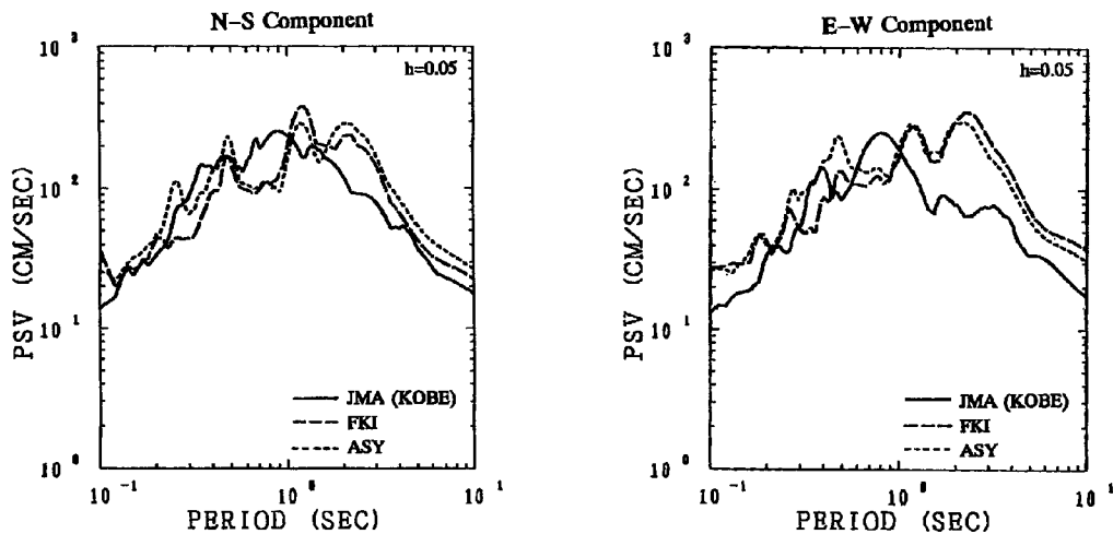
Fig. 25. Comparison of the pseudo velocity response spectra (PVS) of the simulated seismograms at FKI and ASY in seriously damaged areas ranked JMA Intensity 7 and of the observed seismograms at KOB in less damaged area ranked Intensity 6.
