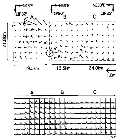
Fig. 13. Distribution of total slip vector (upper) and of moment rate function (lower) obtained from the waveform inversion using strong ground motion records.
