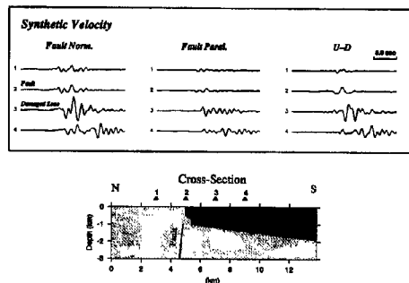
Fig. 19. Synthetic seismograms selected from seismic record section for basin model in Fig. 18. Cross section of assumed model is shown with locations of selected four sites.
