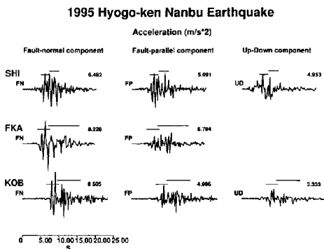
Fig. 6. Observed acceleration waveforms at near-source stations. Left, middle, and right are horizontal fault-normal-component, horizontal fault-parallel-component, and vertical component, respectively.
