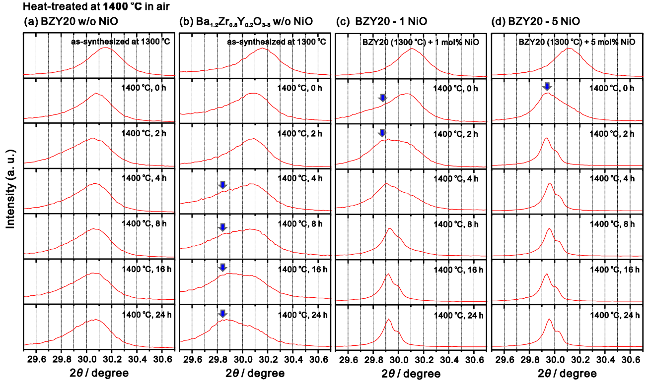
Fig. 9 Variation of (011) diffraction peak shape of (a) BZY20, (b) \text{Ba}_{1.2}\text{Zr}_{0.8}\text{Y}_{0.2}\text{O}_{3-\delta} , (c) BZY20 – 1 NiO, and (d) BZY20 – 5 NiO, which were heat-treated at 1400 °C in air for different time. The samples were finally quenched in ambient atmosphere.
