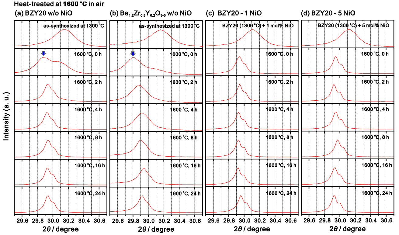
Fig. 8 Variation of (011) diffraction peak shape of (a) BZY20, (b) \text{Ba}_{1.2}\text{Zr}_{0.8}\text{Y}_{0.2}\text{O}_{3-\delta} , (c) BZY20 – 1 NiO, and (d) BZY20 – 5 NiO, which were heat-treated at 1600 °C in air for different time. The samples were finally quenched in ambient atmosphere.
