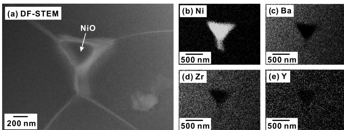
Fig. 2 (a) A DF-STEM image of BZY20 - 5 NiO, which was heat-treated at 1600 °C in air for 24 h, and distribution of (b) Ni, (c) Ba, (d) Zr, and (e) Y by STEM-EDS elemental mapping analysis..
