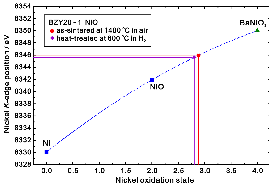
Fig. 14 Nickel oxidation state plotted against Ni K-edge position. Ni K-edge position of tetravalent Ni ( \text{BaNiO}_3 ) was reported by O'Grady et al.[26]. A polynomial of degree two (dash curve) was applied for calibration curve. Examples for determining the oxidation state of Ni in \text{BaZrO}_3 was plotted for example by using the samples of BZY20 – 1 NiO heat-treated at 1400 °C in air for 24 h, and 600 °C in \text{H}_2 for 24 h in sequence.
