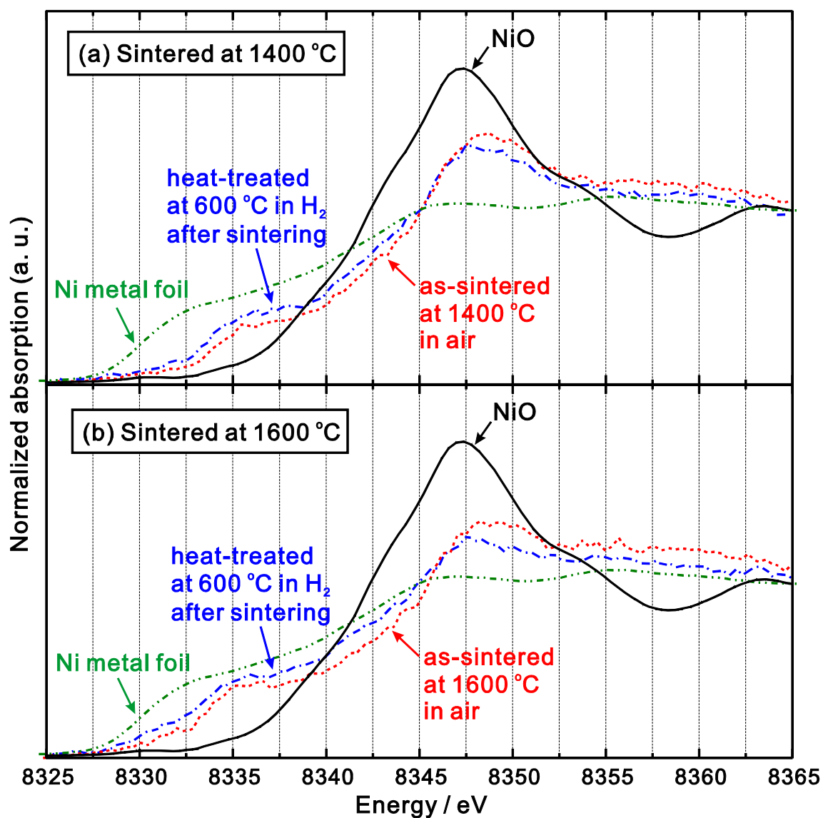
Fig. 13 Ni K-edge XANES data obtained for (a) BZY20 – 1 NiO heat-treated at 1400 °C in air for 24 h, and subsequently heat-treated at 600 °C in H 2 for 24 h, and (b) BZY20 – 1 NiO heat-treated at 1600 °C in air for 24 h, and subsequently heat-treated at 600 °C in H 2 for 24 h. XANES data of Ni and NiO are also plotted. Data were collected at 8 K in vacuum.
