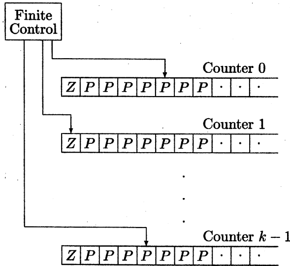
Figure 2: A k -counter machine ( \text{CM}(k) ).
