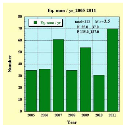
Fig.3 Yearly number of earthquakes M \geq 2.5 in the whole region shown in Fig.1. However, the plotted time is only after 2005, when the extensometers near the Hokuriku observatory started to work.
