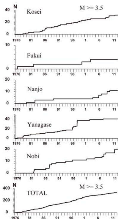
Fig.5 Cumulative nonber of earthquakes for M \geq 3.5 in 5 regions and total area from 1976-Apr., 2012.
