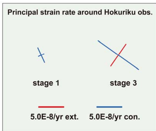
Fig.11 Maximum principal strain calculated from the GPS, named SABAE, FUKUIKEDA, and IMAJOU, from Oct., 2005 to Apr., 2012.
