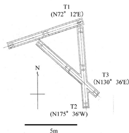
Fig.8 The extensometers set near the Hokuriku observatory. Their lengths are 7m. Observation directions of the instruments are shown in the figure.
