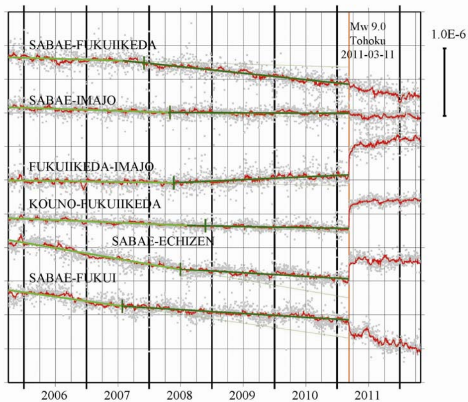
Fig.7 Baseline strain calculated from the GPS output data by the Geospatial Information Authority of Japan.
