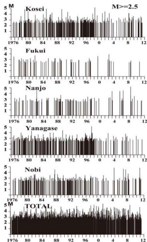
Fig.4 Time-magnitude distribution for M \geq 2.5 earthquakes in 5 regions and total area from 1976-Apr., 2012.
