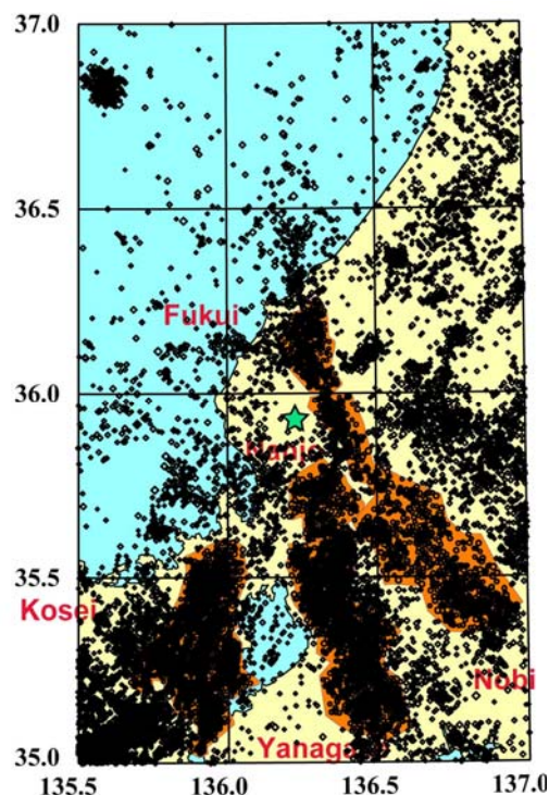
Fig.1 Map of epicenters, Jan., 1976 – Apr., 2012, M \geq 1.5 , D \leq 30\text{km} (brack) Total number equals to 22, 95.★ is the point of Hokuriku Observatory. Five orange regions show the studied areas.
