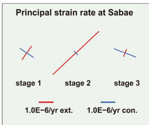
Fig.10 Maximum principal strain calculated from the extensometers in the Hokuriku Observatory tunnel, from Oct., 2005 to Apr., 2012.
