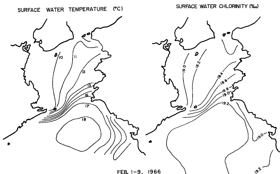
Fig. 2 Distributions of surface water temperature and chlorinity in winter. An oceanic front appears at the mouth of Kii-Suido.
