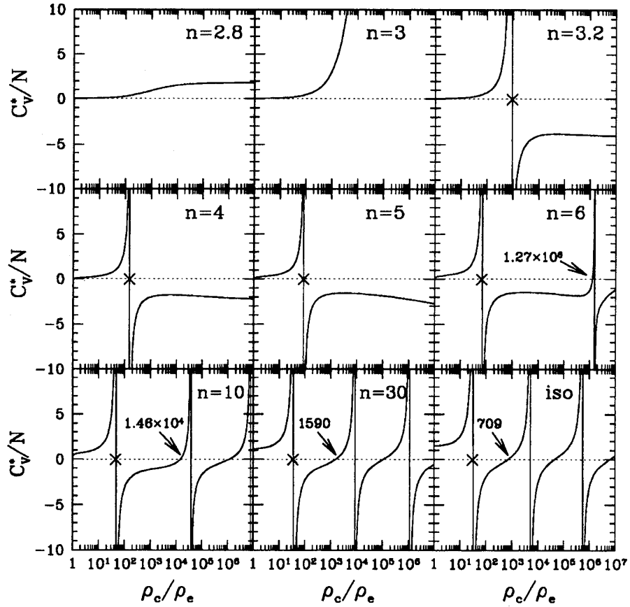
Figure 2: Normalized specific heat per particle C_v^*/N as a function of density contrast \rho_c/\rho_e near the critical polytropic indices n = 3 (upper) and n = 5 (middle), and large n cases(lower). Here, the normalized specific heat C_v^* is defined by C_v/(h^2/GMr_e)^{(3/2)/(n-3/2)} (see Ref.[8] in detail).
