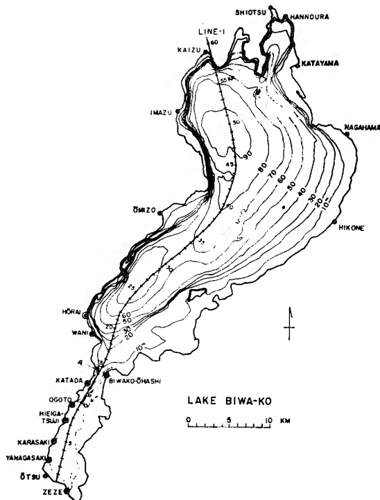
Fig. 1. Bottom topography of Lake Biwa-ko. Longitudinal seiche oscillations are assumed to occur along the solid thick line. Numerals along this line are the length in kilometers from the southern end of the lake. Double black circles show the observation stations.
