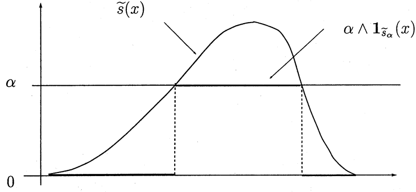
Figure 3: \tilde{s}(x) = \sup_{\alpha \in [0,1]} \{\alpha \wedge \mathbf{1}_{\tilde{s}_\alpha}(x)\} , x \in \mathbb{R}^n
