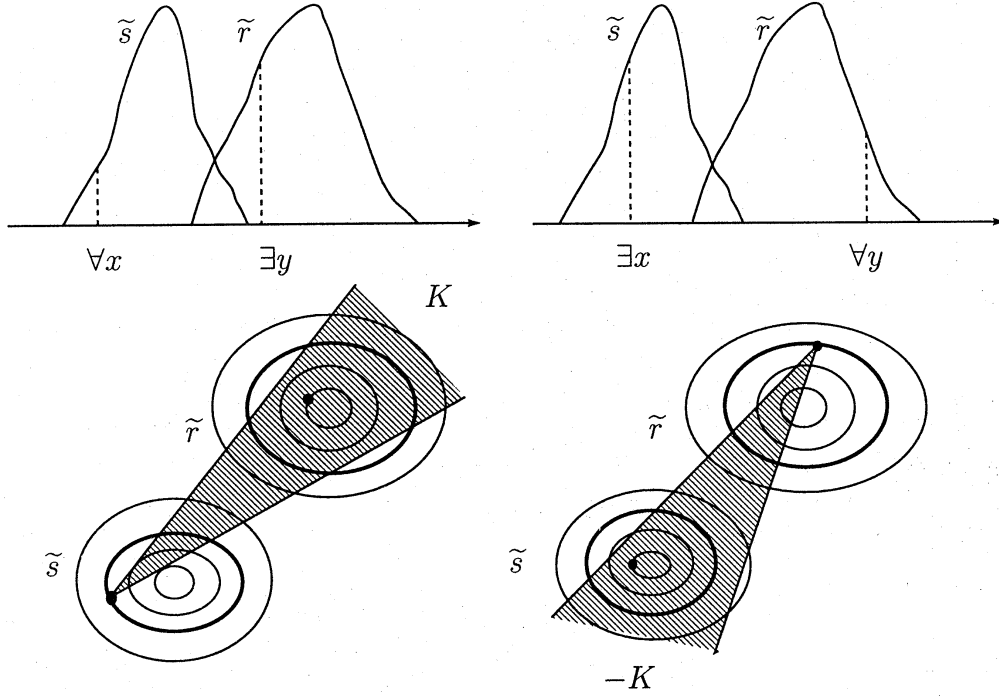
Figure 5: The binary relation \tilde{s} \preccurlyeq_K \tilde{r} on \mathcal{F}(\mathbb{R}) and \mathcal{F}(\mathbb{R}^2)
