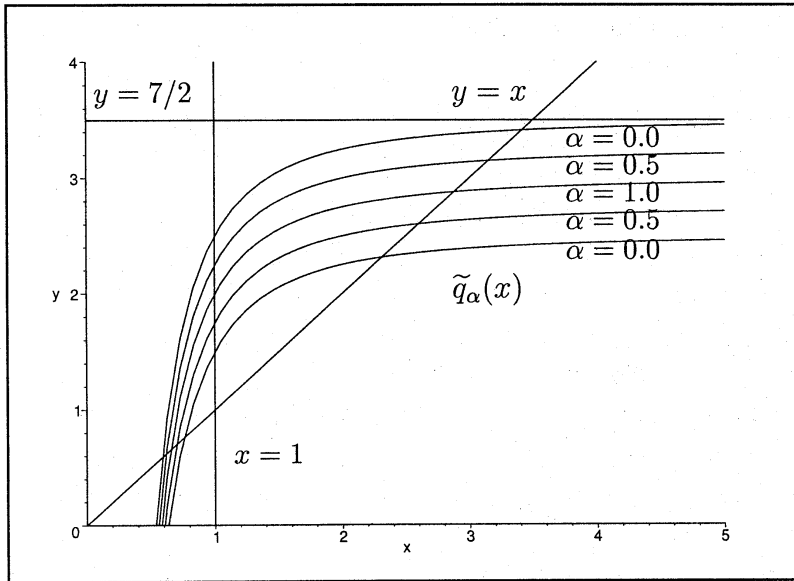
Figure 11: \tilde{q}_\alpha(x) and the limit \tilde{s}(x) of \{\tilde{s}_t(x)\}
