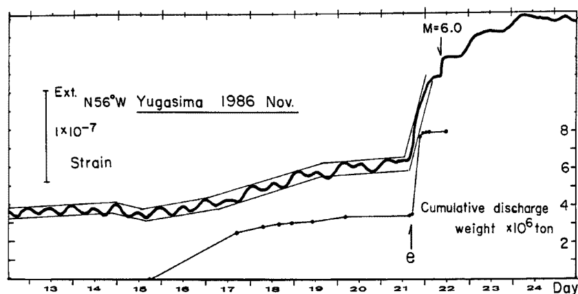
Fig. 6. Strain variation at Yugashima during the eruption of Izu-oshima. (after Umeda et al., 1991)
