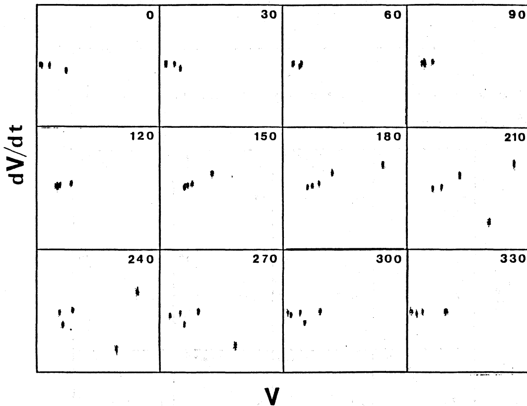
Fig.4 The stroboscopic plots of a 4/5-synchronized oscillation in squid giant axons. The number in each stroboscopic plot shows the corresponding phase(°) of the sinusoidal force.
