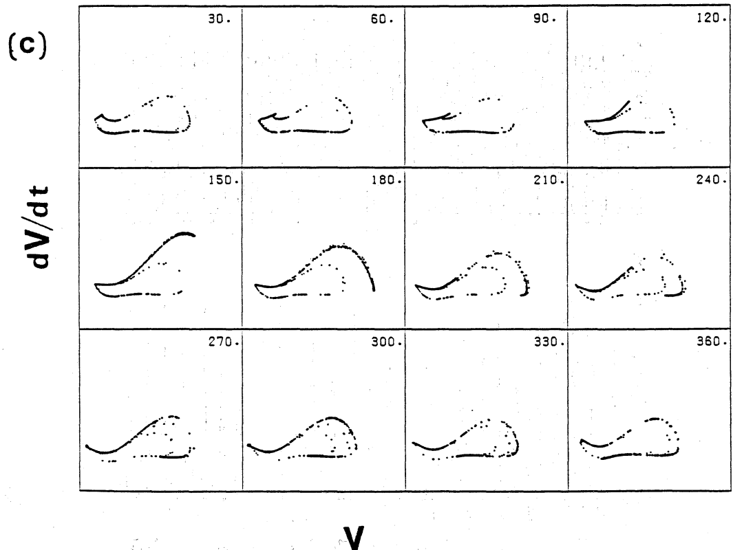
Fig.3 A chaotic oscillation in the H-H eqs. ( A=40.0 \mu A/cm^2 & F=300.0 Hz). (a) The waveforms of the sinusoidal force (above) and the membrane potential (below). (b) The stroboscopic plots on the plane V \times m at each 30^\circ phase of the sinusoidal force. (c) The stroboscopic plots on the plane V \times dV/dt at each 30^\circ degree of the sinusoidal force.
