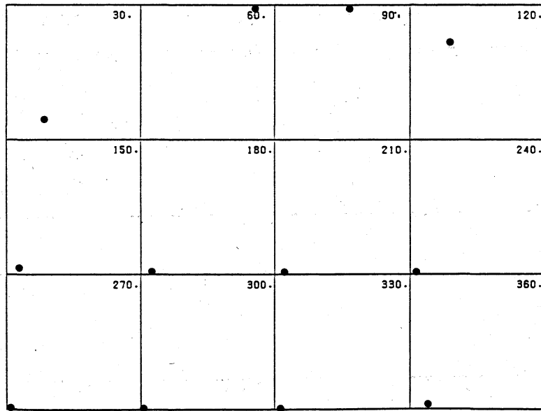
Fig.1 A harmonically synchronized oscillation in the H-H eqs. ( A = 40.0 \mu\text{A}/\text{cm}^2 & F = 100.0 \text{ Hz} ). (a) The waveforms of the sinusoidal force I (above) and the membrane potential V (below). (b) The stroboscopic plots on the plane V (the membrane potential) \times m (the sodium activation) at each 30^\circ phase of the sinusoidal force. The number in each stroboscopic plot shows the corresponding phase ( ^\circ ) of the sinusoidal force.
