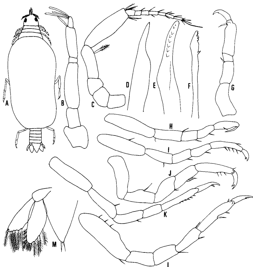
Fig. 2. Gnathia capillatai n. sp (Praniza, parasitic juvenile 8.0 mm long). A: Dorsal view, B: Antennula, C: Antenna, D: paragnath; E: mandible, F: Maxillula, G: Gnathopod; H-L: Pereopods 1-5, M: Telson and Uropod.
