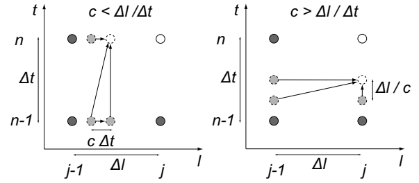
Fig. 1 Multi-step, Multi-reach stabilization method for Muskingum Cunge model
