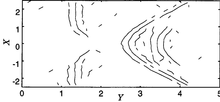
Figure 3.19: Extraction of quasi wavefront p \in G from data s(X, Y) for S/N = 3\text{dB} .
