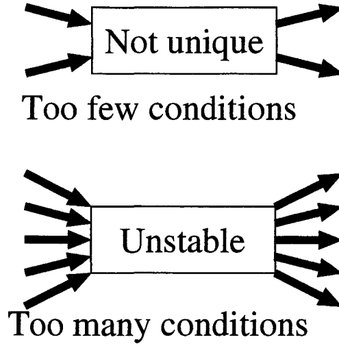
Figure 1.13: Condition number and inverse problem.
