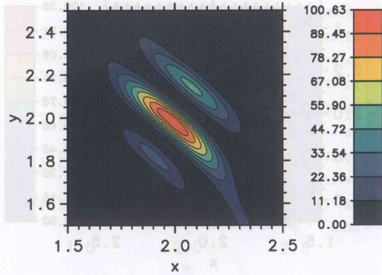
Figure 2.4: Evaluation function with the true filter.
