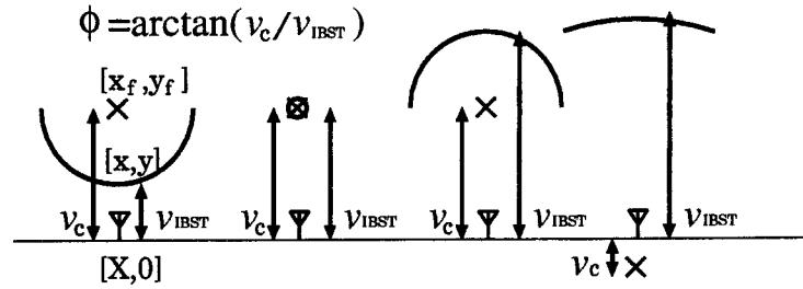
Figure 5.8: Locations of antenna, caustic and target.
