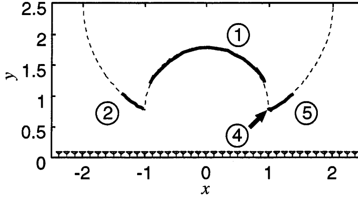
Figure 5.12: Estimated target shape for S/N=20\text{dB} .
