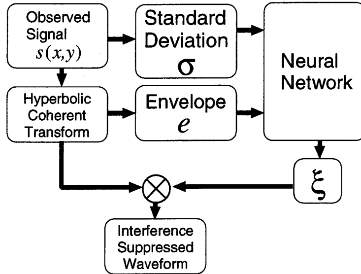
Figure 2.13: The outline of interference suppression in the proposed algorithm.
