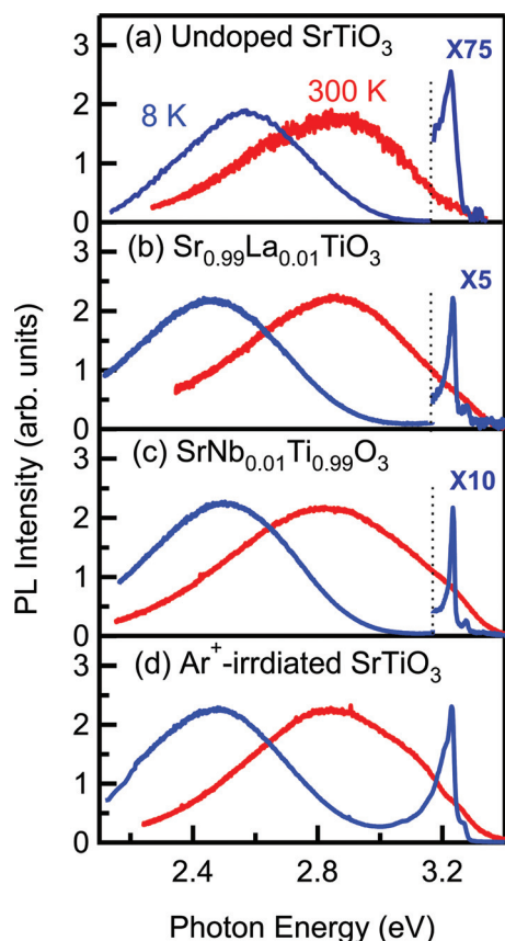
FIG. 1. (Color online) Time-integrated PL spectra of (a) strongly photoexcited undoped \text{SrTiO}_3 , (b) \text{Sr}_{0.99}\text{La}_{0.01}\text{TiO}_3 , (c) \text{SrNb}_{0.01}\text{Ti}_{0.99}\text{O}_3 , and (d) \text{Ar}^+ -irradiated \text{SrTiO}_3 at 8 and 300 K.
