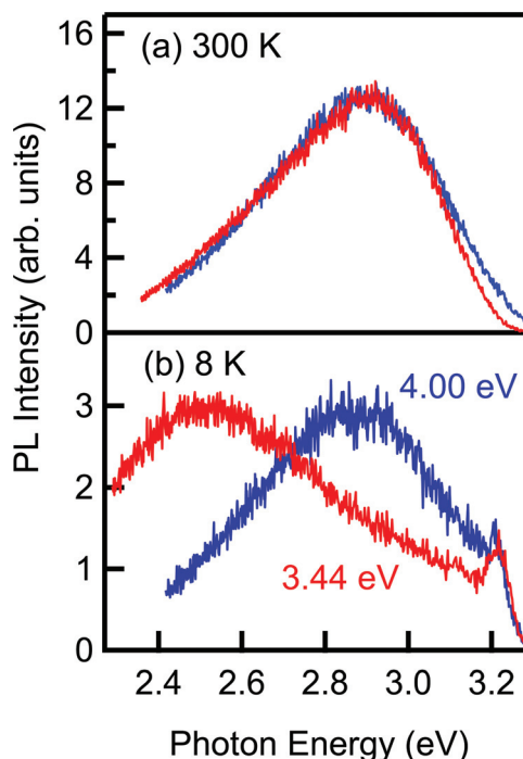
FIG. 2. (Color online) Time-integrated PL spectra of \text{SrNb}_{0.01}\text{Ti}_{0.99}\text{O}_3 excited at 3.44 and 4.00 eV at (a) 300 and (b) 8 K.
