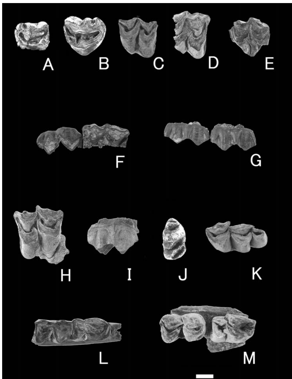
Fig. 9. A-M: Palaeotragus cf. germaini . A) occlusal view of the right P^2 (KNM-SH 37887); B) occlusal view of the right P^3 (KNM-SH 37892); C) occlusal view of the right M^{1 \text{ or } 2} (KNM-SH 37894); D) occlusal view of the right upper molar (KNM-SH 37895); E) occlusal view of the left M^{1 \text{ or } 2} (KNM-SH 37898); F) occlusal and G) buccal views of the left M^{1 \text{ or } 2} (KNM-SH 37888); H) occlusal and I) buccal view of the left M^{1 \text{ or } 2} (KNM-SH 40145); J) occlusal view of the right P_3 (KNM-SH 18005); K) occlusal view of the left M_3 (KNM-SH 37893); L) occlusal view of the left mandible with P_4 - M_1 (KNM-SH 37900); M) occlusal view of the right mandible with P_4 - M_1 (KNM-SH 37891). Scale in cm.
