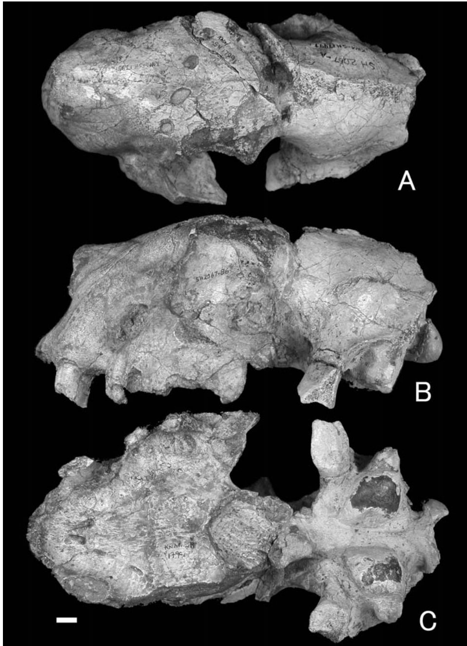
Fig. 2. A-C: Machairodontinae gen. et sp. indet. A) dorsal, B) left lateral and C) ventral view of the skull (KNM-SH 17991). Scale in cm.
