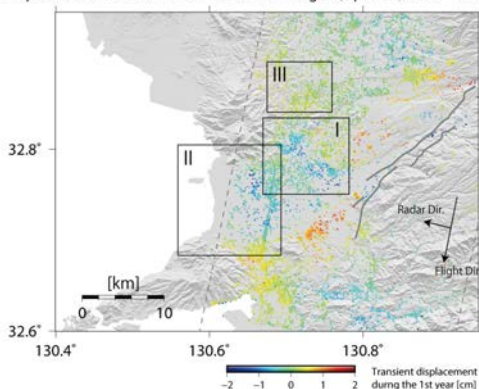
Transient displacement from ALOS-2/PALSAR-2 images (April 18, 2016–December 10, 2018)
