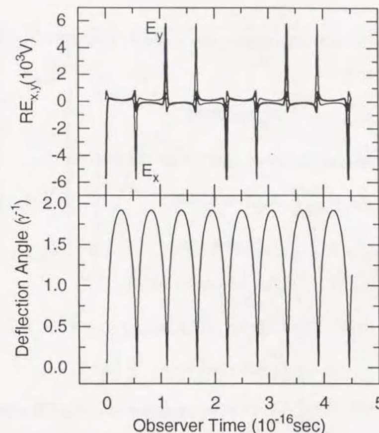
Figure 7.4. Electric field obtained from the rhombus undulator and the deflection angle.
