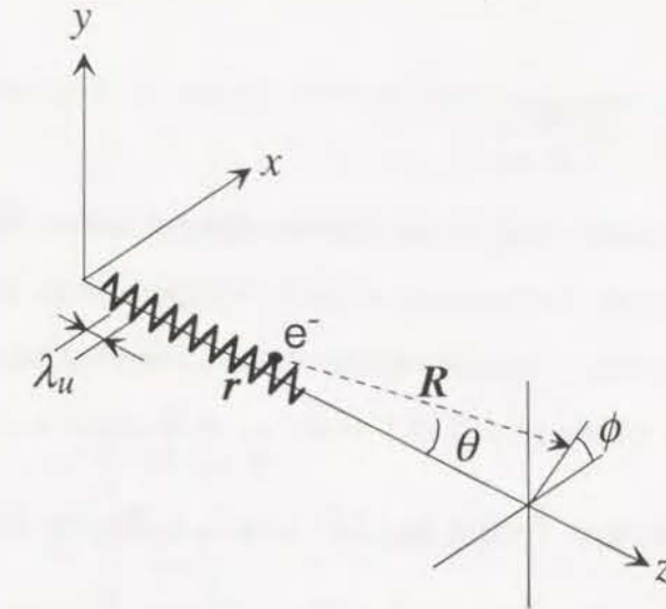
Figure 2.3. ID with arbitrary fields.
