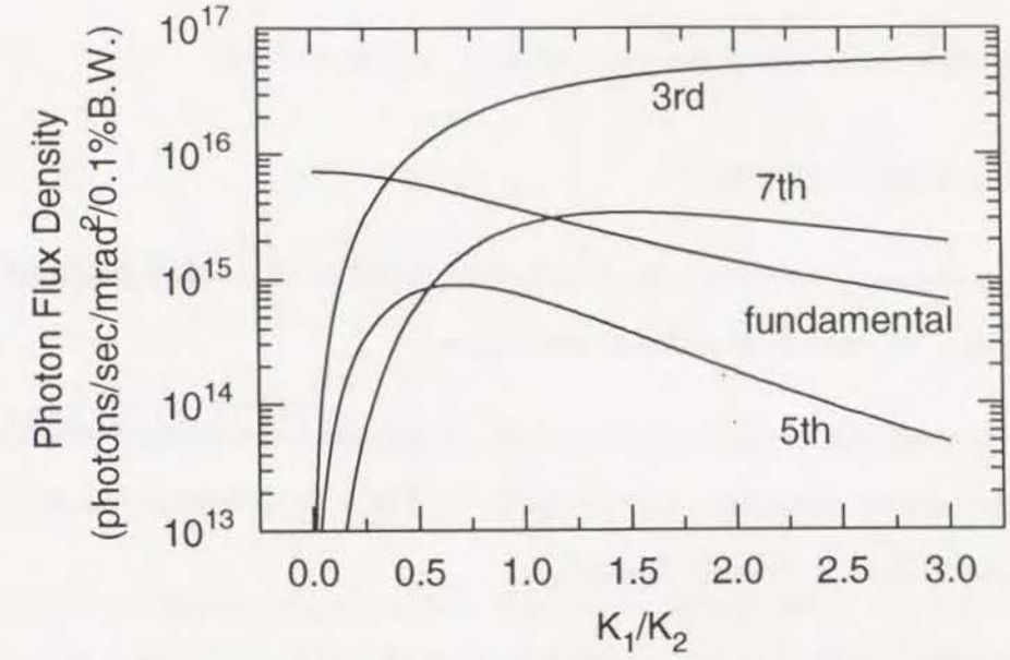
Figure 7.5. K-ratio dependence of the photon flux density.
