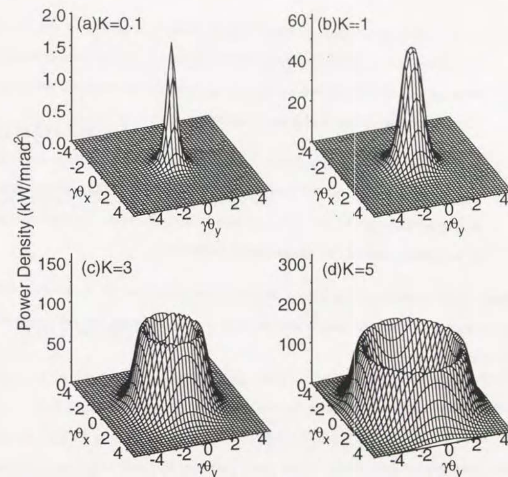
Figure 2.14. Examples of the spatial distribution of the power density obtained from the helical undulator.
