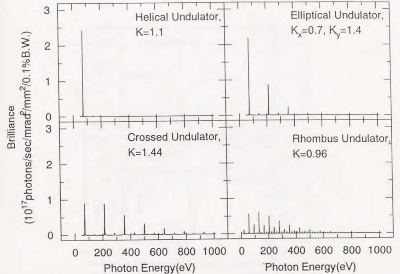
Figure 6.3. Examples of spectra obtained from the (a) helical, (b) elliptical, (c) crossed and (d) rhombus undulators.
