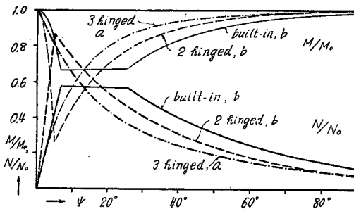
Fig. 12 The comparison among M/M_0 , N/N_0 versus \psi diagrams in built-in, 2 hinged and 3 hinged arches carrying a concentrated load at the centre of span ( h/L=0.1 )
